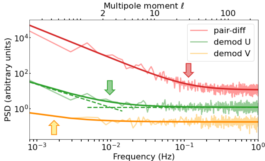
Figure 1: Spectra of 40 GHz data from one 3-hour segment, arbitrarily scaled and offset for visual clarity. Spectra are modeled as white noise plus a power law (dashed lines for demodulated- U ). The knee frequency is where these components are equal (colored arrows). Demodulation significantly lowers the knee frequency compared to pair differencing alone, enabling access to the largest scales (lowest \ell , top axis).
