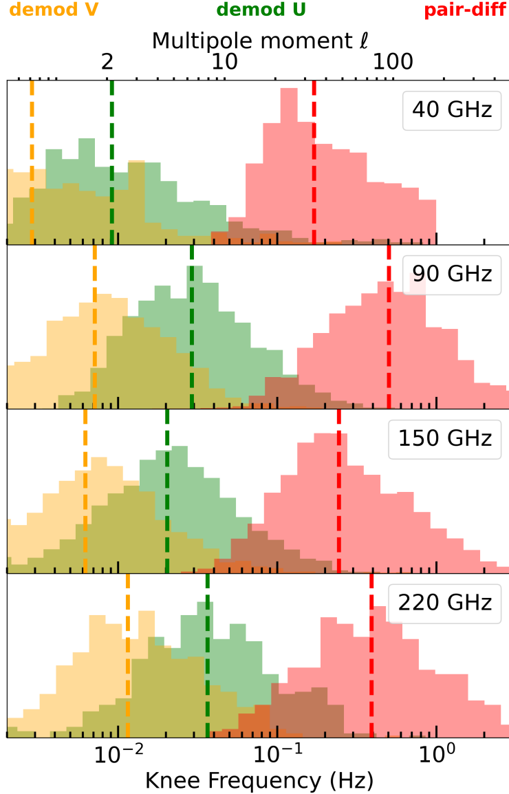
Figure 2: Distribution of knee frequencies for all four CLASS observing bands, for pair-differenced (red), demodulated- U (green), and demodulated- V (yellow). Medians of each distribution as denoted by vertical dashed lines.
