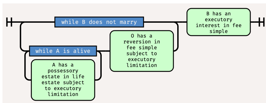
Figure 3: Littleton output
