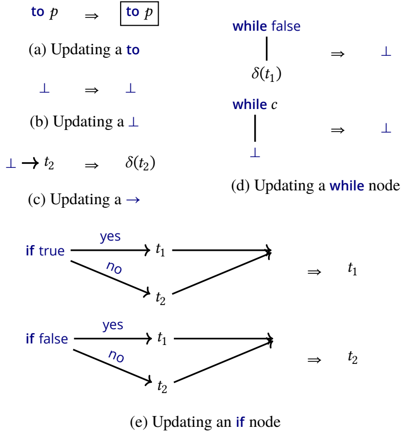
Figure 22: Update rules
