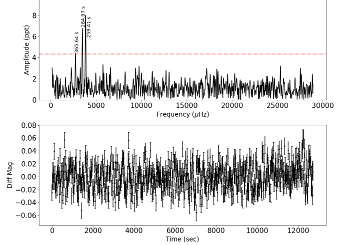
Figure 5. FT and light curve, top and bottom panel respectively, for TIC 20979953 based on data obtained from the Pico dos Dias observatory on 2020-06-14. The data spans for 3.4 h, with an integration time of 17 s.
