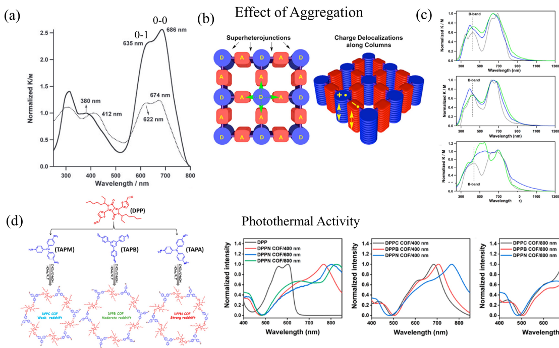
Fig. 2 (a) H- and J- type bands observed in UV-vis absorption of NiPc COF (solid black). Although referred to as H-aggregates, the ratio of the intensities of the vibronic peaks I_{0-0}/I_{0-1} is greater in NiPc COF compared to the (\text{MeO})_8\text{PcNi} monomer (dotted black) suggesting J-type aggregation 257 (copyright 2011 John Wiley & Sons, Inc). (b) Schematic of segregated bicontinuous \pi -columnar arrays observed in COFs. 258 (c) UV-vis observation observed in \text{DMP}_C\text{-A}_{\text{DI}} COFs also display H- and J- type signatures in the UV-vis. 258 (d) UV-vis absorption of DPP-based donor-acceptor COFs directly correlates with the COF particle size. 47 Figs. b,c reprinted with permission from Ref. 258. Copyright 2015 American Chemical Society, Fig. d reprinted with permission from Ref. 47. Copyright 2021 American Chemical Society
