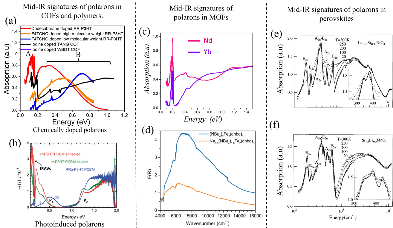
Fig. 8 (a) Mid-IR signatures of “bound” polarons in chemically doped polymers 230,231 and COFs 64,216 using data from Refs. 216,230,231. A red shift of the high energy peak B signifies enhanced polaron delocalization. (b) Mid-IR signatures of photoinduced polarons in conjugated polymers. 324,325 (c,d) Mid-IR signatures of polarons in MOFs. 326,327 Fig. c replotted from Ref. 326. Fig. d reprinted with permission from Ref. 327. Copyright 2015 American Chemical Society (e,f) Mid-IR signatures of polarons in perovskites. 328 Copyright 1996 by American Physical Society. All rights reserved.
