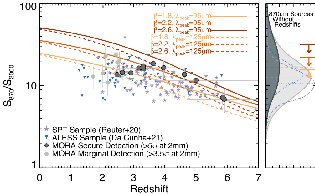
Figure 11. The 870 \mu\text{m} to 2 mm flux density ratio against redshift and in histogram for DSFGs from various samples. Left: the S_{870}/S_{2000} ratio for DSFGs that have secure redshift constraints, including >5\sigma MORA sources (dark gray points) and marginal MORA sources (light gray points); we have also overplotted two other samples of well-characterized DSFGs in the literature: the SPT (1.4 mm selected) sample from Reuter et al. (2020), and the ALESS (870 \mu\text{m} selected) sample from da Cunha et al. (2021). Overlaid are tracks of specific SEDs with variable dust temperature ( \lambda_{\text{peak}} = 95 \mu\text{m} or 125 \mu\text{m} , solid vs. dashed) and variable emissivity spectral index ( \beta = 1.8, 2.2 , or 2.6 , in increasingly dark shades of orange, respectively). Right: histograms of S_{870}/S_{2000} for sources without redshifts that have 870 \mu\text{m} ALMA data (dark gray), sources with 870 \mu\text{m} data only from SCUBA-2 (light gray), and the full distributions of the SPT sample (purple dotted-dashed) and ALESS sample (dotted blue). Downward arrows mark the maximum color ratio that could correspond to a given value of \beta at z = 2.5 ; higher ratios are not allowed for the given \beta , as the ratio of flux densities only diminishes with redshift. Our data suggest a range of \beta values apply to this sample, from some being fully consistent with the often-presumed value of \beta = 1.8 , to some being more consistent with steeper slopes, \beta \approx 2.2\text{--}2.6 .
