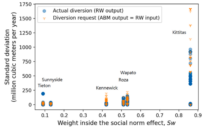
Fig. 7. Standard deviations of 465 LSA simulation results with respect to calibrated Coupled-YAKRW outputs. The x-axis is the weight inside the social norm effect. Blue circles represent actual diversion (RW output), and orange triangles indicate diversion requests sent from ABM to RW (RW input).
