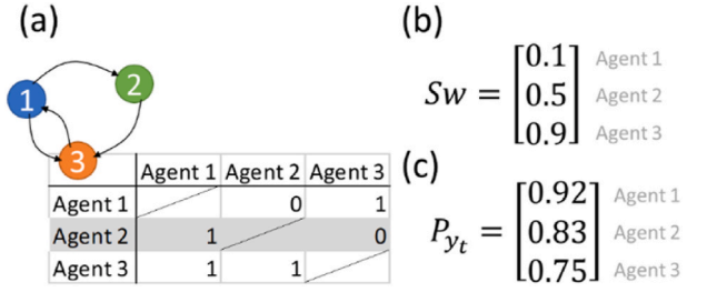
Fig. 3. (a) S is a social network matrix. Each row of the matrix is the social network of the agent in that row, which is affected by the agent in the column with cell's value 1. (b) Sw is a weight vector to balance between neighbor opinions and the agent's own beliefs. (c) P_{y_t} is a collection of agent's evaluations of water supply conditions in y_t .
