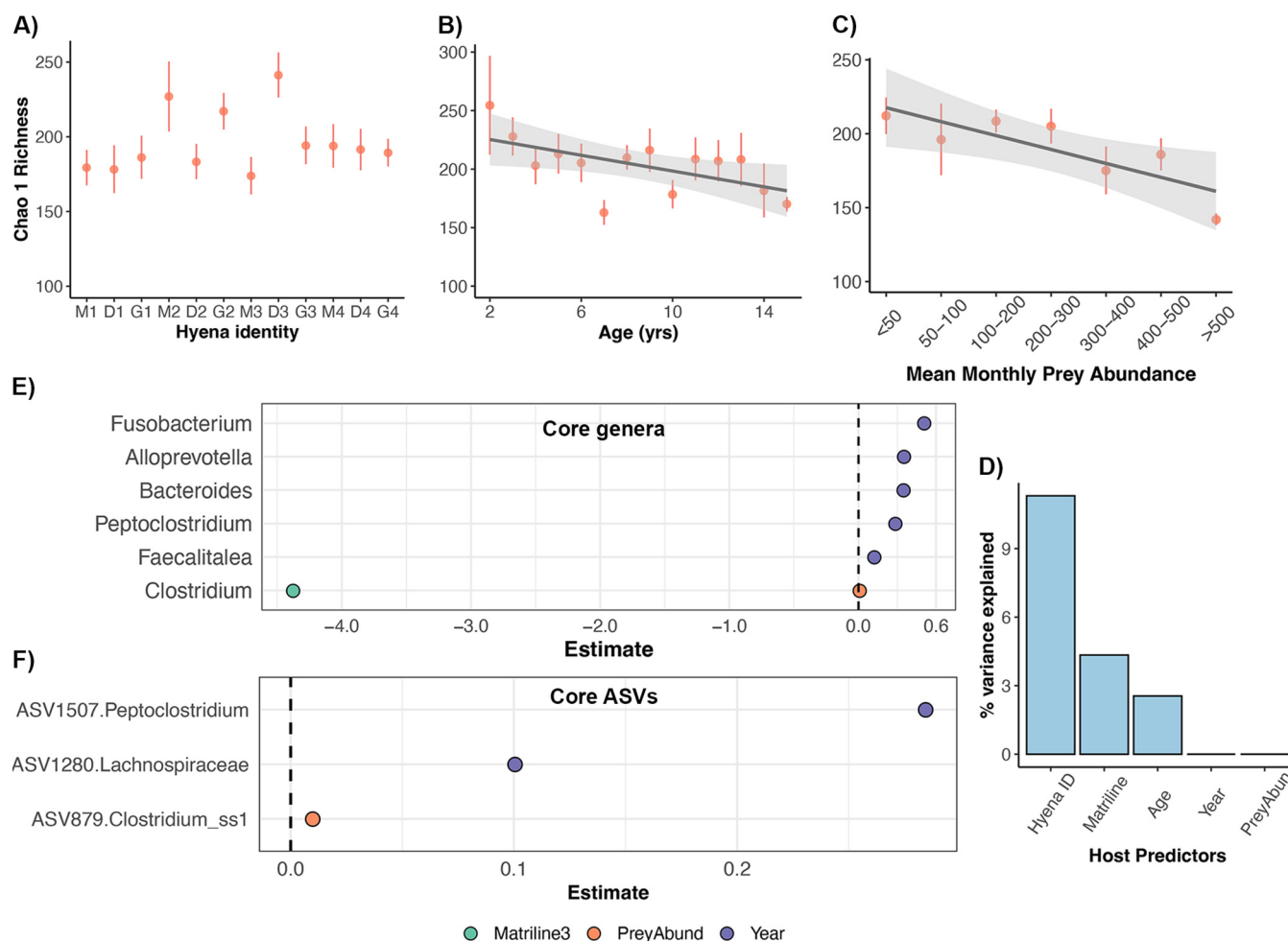
FIG 2 Socioecological predictors of the gut microbiome in wild spotted hyenas. (A to C) Plots of microbiome Chao 1 richness (mean \pm SE) for each hyena individual (A), age category (B), or mean monthly prey abundance (C) for 16S rRNA gene data. The shaded lines with a 95% confidence interval (CI) represent the relationship between x and y , estimated as a linear regression. See Data Set S1 in the supplemental material for statistical output from the linear models. (D) Plots of R^2 values from PERMANOVA models testing whether host individual identity, matriline, age, mean monthly prey abundance, and sample year predicted gut microbiome beta-diversity (for 16S rRNA gene data). See Table 2 for exact model output. (E and F) Plots of beta-coefficients from linear mixed models regressing the abundance of core genera (E) or ASVs (F) against the five host predictors listed above. Each point represents a beta-coefficient and is color coded by host predictor. If a beta-coefficient is positive, the abundances of that bacterial taxon were positively correlated with the host predictor. Only beta-coefficients with P values of <0.05 after correcting for multiple comparisons are displayed.
