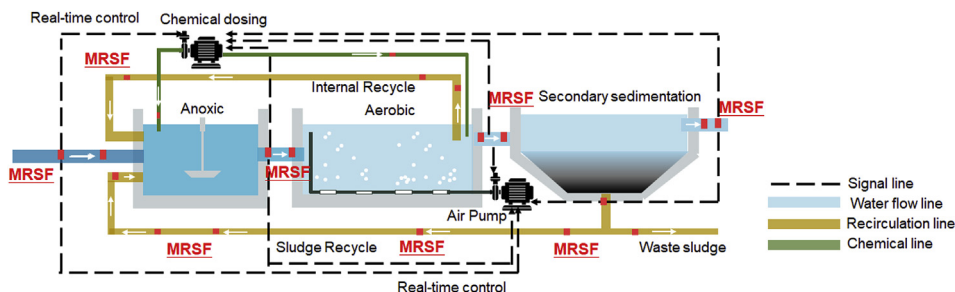
Fig. 9. Diagram of high resolution MRSF monitoring and swift control of each treatment unit in an anoxic/aerobic WWTP.
