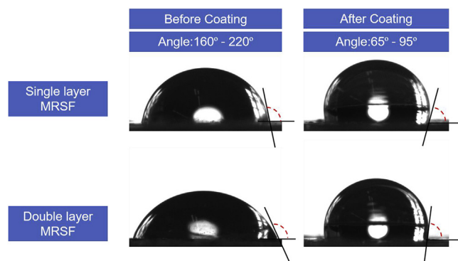
Fig. 8. Contact angle of single-film and double-film MRSFs before and after the silicon glue coated on the sensor surface. (For interpretation of the references to colour in this figure legend, the reader is referred to the Web version of this article.)
