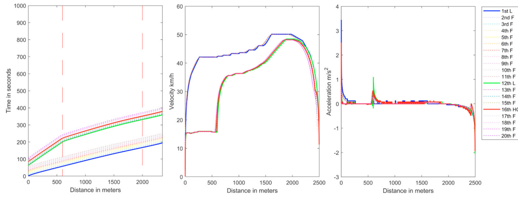
Fig. 3. Eco-driving trajectory planning of heterogeneous platoon in Scenario I. The average traveling time for this scenario is 234.86 s/veh and the maximum velocity in the platoon is below 51 km/h.
