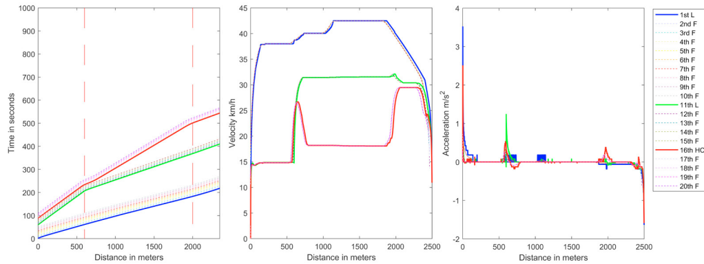
Fig. 4. Eco-driving trajectory planning of heterogeneous platoon in Scenario II. The average traveling time for this scenario is 305.85 s/veh and the maximum velocity in the platoon is about 42.5 km/h.
