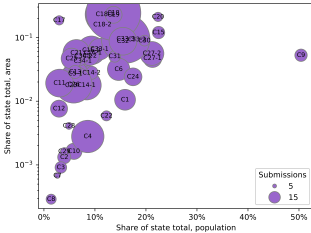
Figure 5: Population share of each cluster in Michigan (plotted on log scale) compared to its share of the statewide area. Circles are sized according to the number of total submissions in each cluster.
