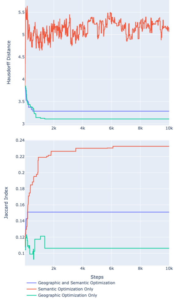
Figure 4: Trace plots of geographic and semantic similarity scores over time with \beta = 10 in the Grand Rapids geocluster in Michigan.
