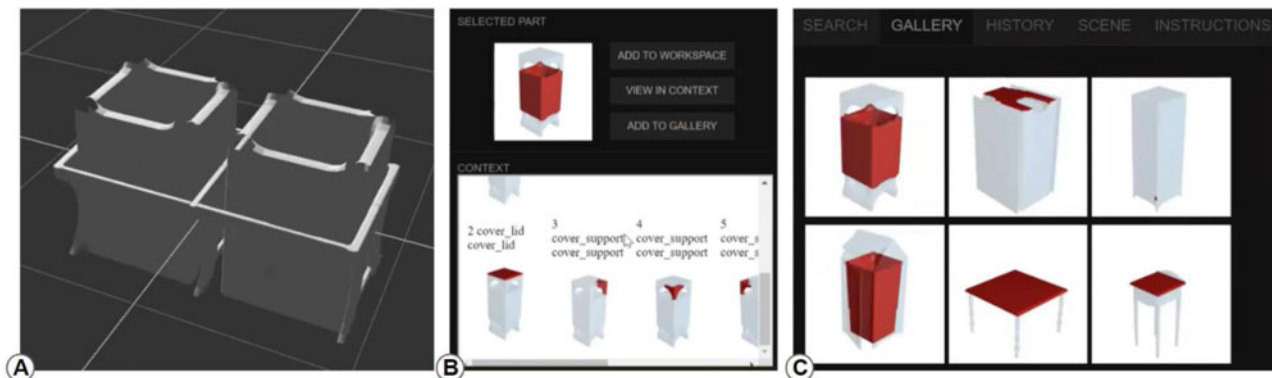
Fig. 3. Interactions with selected part in Figure 2 – (a) adding part to the workspace; (b) viewing part in context by seeing related parts with text labels in the same object assembly; and (c) adding part to a gallery of saved 3D parts.
