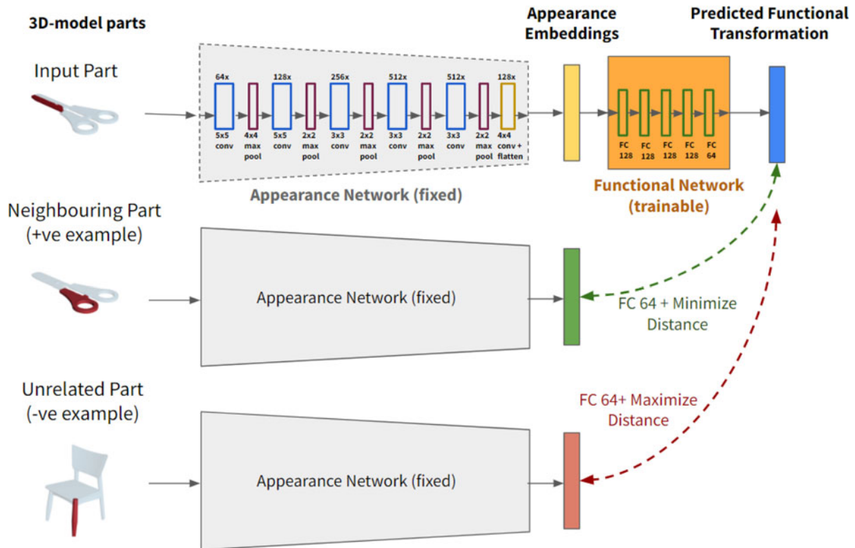
Fig. 1. Overview of process of transformation of embeddings from appearance network to functional embeddings. Appearance embeddings of input part (scissor blade) were used to generate a predicted functional transformation using the functional network. Functional network was then trained by considering this prediction as similar to the appearance embedding of a neighbouring part (scissor handle) and dissimilar to the appearance embedding of an unrelated part (chair leg). Intermediate representation within the functional network was used as the functional embedding of each model part in the dataset.
