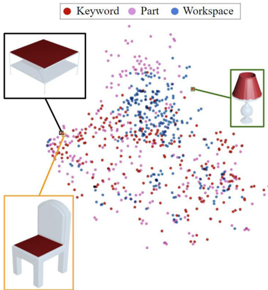
Fig. 7. 2D visualization of the 128-dimensional appearance-based neural network: parts retrieved during the study using each search modality are represented based on their appearance embeddings. Closely related (yellow, chair seat) and distantly related (green, lamp shade) examples in appearance to the reference part (black, tabletop) are shown.
