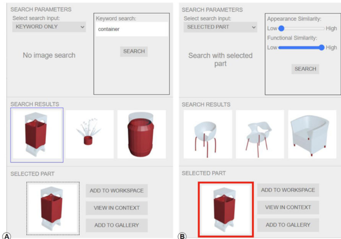
Fig. 2. (a) Search results for a keyword search of the term "container"; (b) search results for a part search of a result from keyword search for "container".
