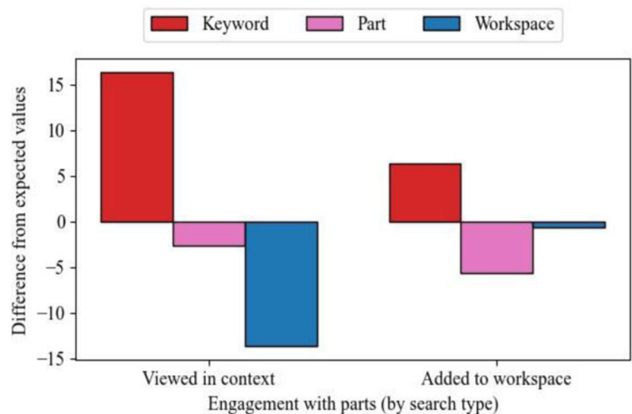
Fig. 6. Differences between the observed and expected values of parts viewed in context and added to the workspace, shown by search type.
