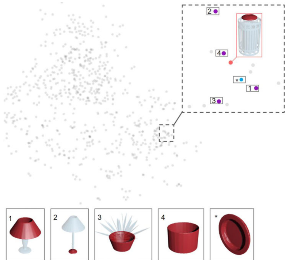
Fig. 8. Expanded view of a cluster of parts in the 2D visualization of the appearance-based neural network. Parts 1–4 are the top 4 nearest neighbors in Euclidean distance to a trash can lid in the full 128-dimensional embedding space. Part * is close based on visual inspection to the trash can lid in the 2D projection.
