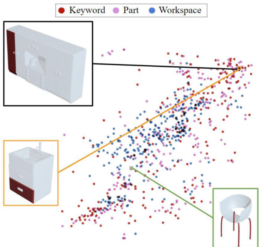
Fig. 9. 2D visualization of the 64-dimensional function-based neural network: parts retrieved during the study using each search modality are represented based on their functional embeddings. Closely related (yellow, sink drawer face) and distantly related (green, chair legs) examples in function to the reference part (black, cabinet door) are shown.
