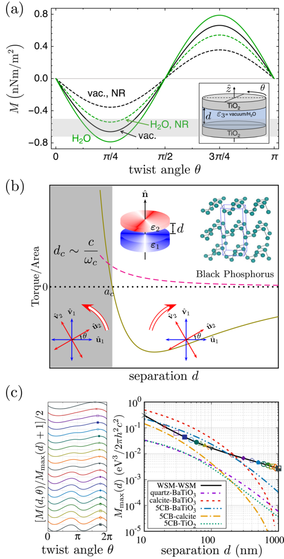
Fig. 3. (Color online) Predictions for the Casimir torque. (a) Casimir torque between \text{TiO}_2 plates with water or vacuum as the intervening dielectric medium at a separation of 30 nm (taken from Ref. 28). The green (black) lines correspond to the results for water (vacuum). The dashed lines are results in the nonretarded limit (NR) and the solid lines take retardation into account. (b) Distance-dependent sign reversal of the Casimir torque (taken from Ref. 29). The solid line shows the Casimir torque between two black phosphorus surfaces (see inset) at the relative angle \theta = \pi/4 . The dashed curve corresponds to the result in the nonretarded limit. (c) Chiral-anomaly-driven Casimir torque between Weyl semimetals (taken from Ref. 30). Left: Normalized Casimir torque as a function of twist angle \theta for various separations. The labels mark the maximum value of the torque, which is used on the figure on the right. Right: Maximal Casimir torque as a function of separation. The result between two Weyl semimetals is depicted as the black line. The dashed lines correspond to the Casimir torque between various birefringent materials. All results are calculated at zero temperature.
