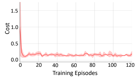
Figure 3: Normalized energy cost during training for our approach with all techniques included for the lightweight building with weather data from Riverside.
