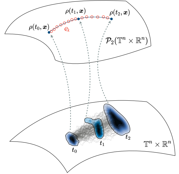
Fig. 3. A schematic of approximating the flow of the joint PDF trajectory \rho(t, \mathbf{x}) via the sequence \{\varrho_k\}_{k \in \mathbb{N}} generated by a variational recursion over \mathcal{P}_2(\mathbb{T}^n \times \mathbb{R}^n) . The curve \rho(t, \mathbf{x}) solves a kinetic Fokker-Planck PDE initial value problem. Points on this curve (shown as three filled circled markers at three specific instances t_0, t_1, t_2 ) are joint PDFs. While the joint PDFs are supported over the finite dimensional base manifold \mathbb{T}^n \times \mathbb{R}^n , the proximal updates \{\varrho_k\}_{k \in \mathbb{N}} (shown as circled markers with no face-color) evolve over the infinite dimensional manifold \mathcal{P}_2(\mathbb{T}^n \times \mathbb{R}^n) .
