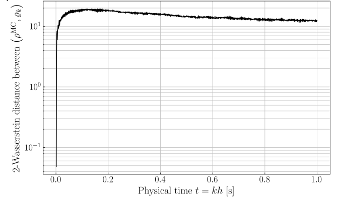
Fig. 14. The 2-Wasserstein distance between the empirical joint PDF (i.e., Monte Carlo estimate) \rho^{\text{MC}} , and the proximal update \varrho^k obtained using the proposed proximal algorithm, for the simulation set up in Sec. V-B.
