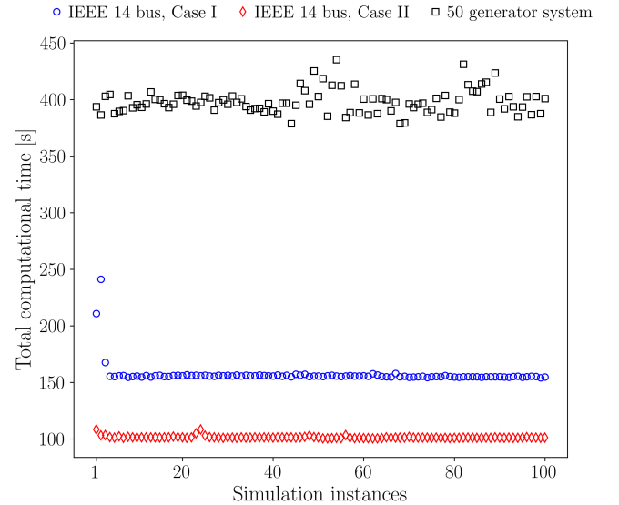
Fig. 10. The total computational times for propagating the transient joint state PDFs over [0, 1 \text{ min}] for the simulation set up in Sec. V-A and Sec. V-B. In each case, we show the total computational time for 100 different simulation instances.
