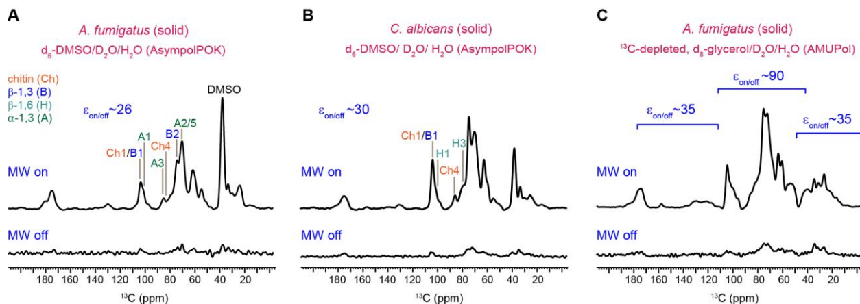
Figure 2: Sensitivity enhancement by MAS-DNP on unlabeled fungal materials. 1D ^{13}\text{C} spectra of unlabeled fungal samples were shown for (A) A. fumigatus solid culture (mainly conidia) and (B) C. albicans solid culture (mainly yeast form) prepared using \text{d}_6\text{-DMSO}/\text{D}_2\text{O}/\text{H}_2\text{O} with 20 mM AsympolPOK. The spectra collected with and without microwave (MW) radiation were compared to give the enhancement factor ( \epsilon_{\text{on/off}} ). (C) 1D ^{13}\text{C} spectra of unlabeled cell walls of A. fumigatus solid culture (mainly conidia) in ^{13}\text{C} -depleted, \text{d}_8\text{-glycerol}/\text{D}_2\text{O}/\text{H}_2\text{O} matrix with 10 mM AMUPol radical. This sample has different enhancement factors for carbohydrate ( \epsilon_{\text{on/off}} \sim 90 ) and protein and lipids ( \epsilon_{\text{on/off}} \sim 35 for aliphatic, aromatic, and unsaturated carbons).
