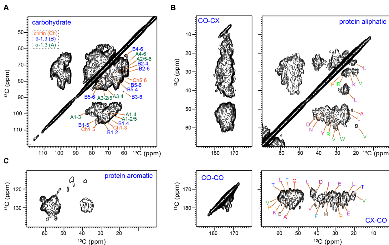
Figure 4: DNP-enabled 2D correlation spectra of unlabeled A. fumigatus solid culture (mostly conidia). Selected regions of DQF 2D dipolar ^{13}\text{C} - ^{13}\text{C} correlation spectra are shown for (A) carbohydrates,
