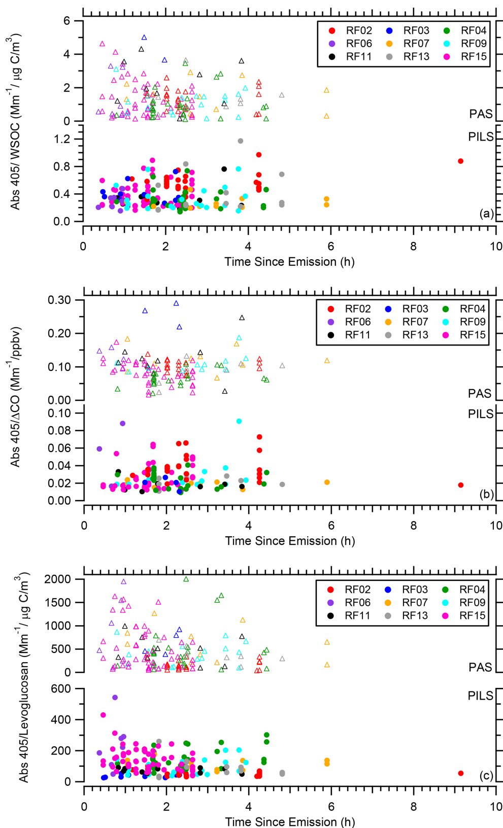
Figure 10. (a) Abs 405 / WSOC, (b) Abs 405 / \Delta\text{CO} , and (c) Abs 405 / levoglucosan as a function of time since emission for all WE-CAN flights with the data segregated by flight. In each plot the PAS total Abs 405 BrC is on top and the PILS water-soluble Abs 405 on the bottom.
