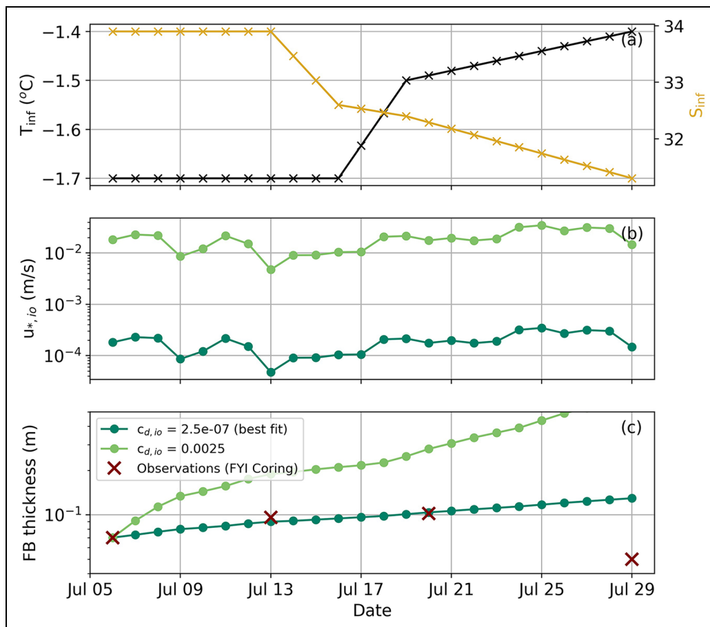
Figure 11. One-dimensional growth and evolution model predictions at the FYI coring site, July 6–29, 2020.
