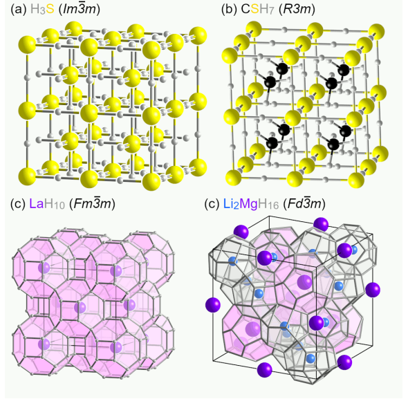
Fig. 6 Selected high-temperature superconducting hydrides that have been calculated to be stable or metastable at high pressures: (a) Im\bar{3}m \text{H}_3\text{S} , the first high-temperature superconducting hydride that was synthesized, [11, 280] (b) R3m \text{CSH}_7 , one example of a predicted ternary superconducting hydride, [87] (c) \text{LaH}_{10} , the first clathrate-like superhydride to be made, [15, 16] and (d) \text{Li}_2\text{MgH}_{16} , a predicted ternary superhydride with an immensely high predicted T_c of 473 K [141]
