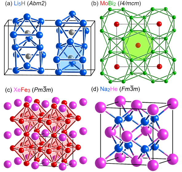
Fig. 4 Examples of strange stoichiometries that arise in compressed materials: (a) predicted \text{Li}_5\text{H} ( Abm2 ) built from \text{Li}_8\text{H} subunits that behave as superalkali atoms, [169] (b) synthesized \text{MoBi}_2 in the \text{CuAl}_2 type, with square antiprisms of Bi containing Mo atoms, [133] (c) synthesized Pm\bar{3}m phase of \text{XeFe}_3 , [217, 218] and (d) synthesized Fm\bar{3}m \text{Na}_2\text{He} , an insulating electride phase. [219]
