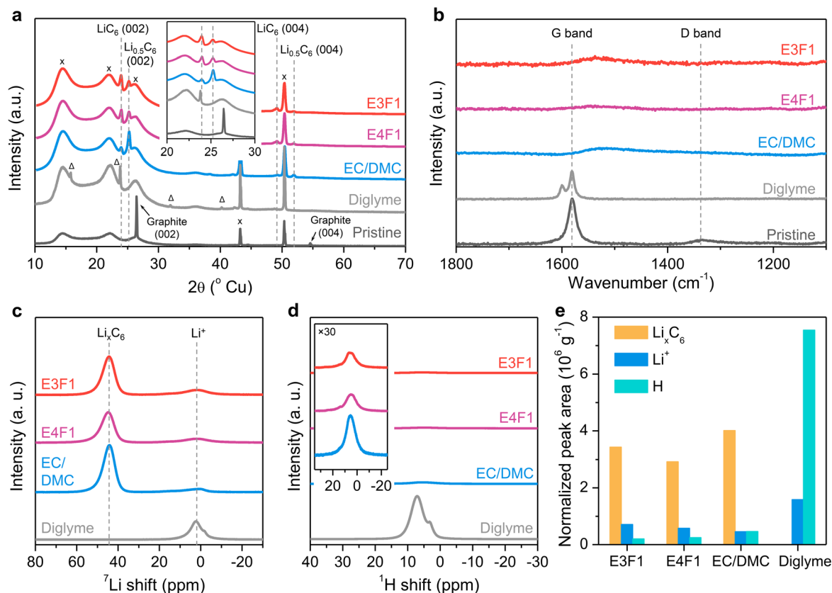
Fig. 3 Ex situ characterization of intercalated graphite. Characterizations of graphite electrodes intercalated in 1 M LiFSA in E3F1 (E3F1), 1 M LiFSA in E4F1 (E4F1), 1 M LiPF 6 in EC/DMC (EC/DMC) and 1 M LiFSA in diglyme (diglyme) electrolytes. (a) XRD patterns of intercalated graphite with pristine graphite as control. x: background peaks from copper and polyimide substrates; Δ: (002), (003), (004) and (005) peaks of ternary GIC (from left to right). The inset shows an enlarged view of the region from 2\theta = 20^\circ to 30^\circ . (b) Raman spectra of intercalated graphite with pristine graphite as control. (c–e) Solid state MAS NMR of intercalated graphite: (c) ^7\text{Li} NMR spectra; (d) ^1\text{H} NMR spectra (the inset shows spectra magnified 30 times); (e) normalized peak integrations. NMR spectra intensity and peak integrations were normalized by number of scan and sample mass.
