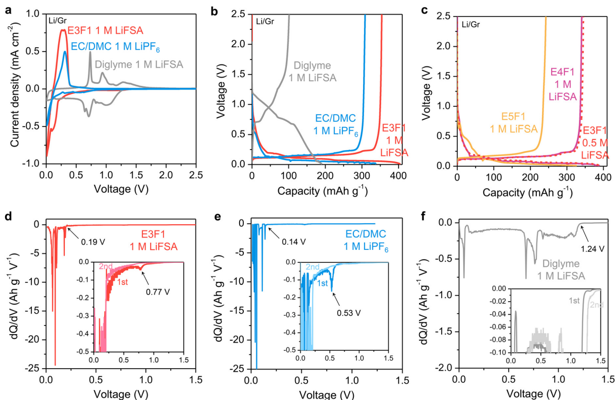
Fig. 2 Electrochemical performance in half cells. (a) Cyclic voltammetry of lithium/graphite (Li/Gr) cells using 1 M LiFSA in E3F1, 1 M LiFSA in diglyme and 1 M LiPF 6 in EC/DMC as electrolytes at a scan rate of 0.05 mV s -1 from open circuit voltage to 0.01 V and then reverse scanned to 2.5 V. (b and c) The first galvanostatic cycle of Li/Gr half cells at a current rate of C/20 (1C ≈ 2.17 mA cm -2 ). (d) Voltage profiles of Li/Gr cells using 1 M LiFSA in E3F1, 1 M LiFSA in diglyme and 1 M LiPF 6 in EC/DMC. (e), Voltage profiles of Li/Gr cells using 1 M LiFSA in E4F1, 1 M LiFSA in E5F1 and 0.5 M LiFSA in E3F1. (d–f) First-order derivatives of the first cycle graphite intercalation voltage profiles in Li/Gr cells using (d) 1 M LiFSA in E3F1, (e) 1 M LiPF 6 in EC/DMC and (f) 1 M LiFSA in diglyme. The insets in (d–f) are enlarged views with the differential curves of both the first and second intercalation for comparison.
