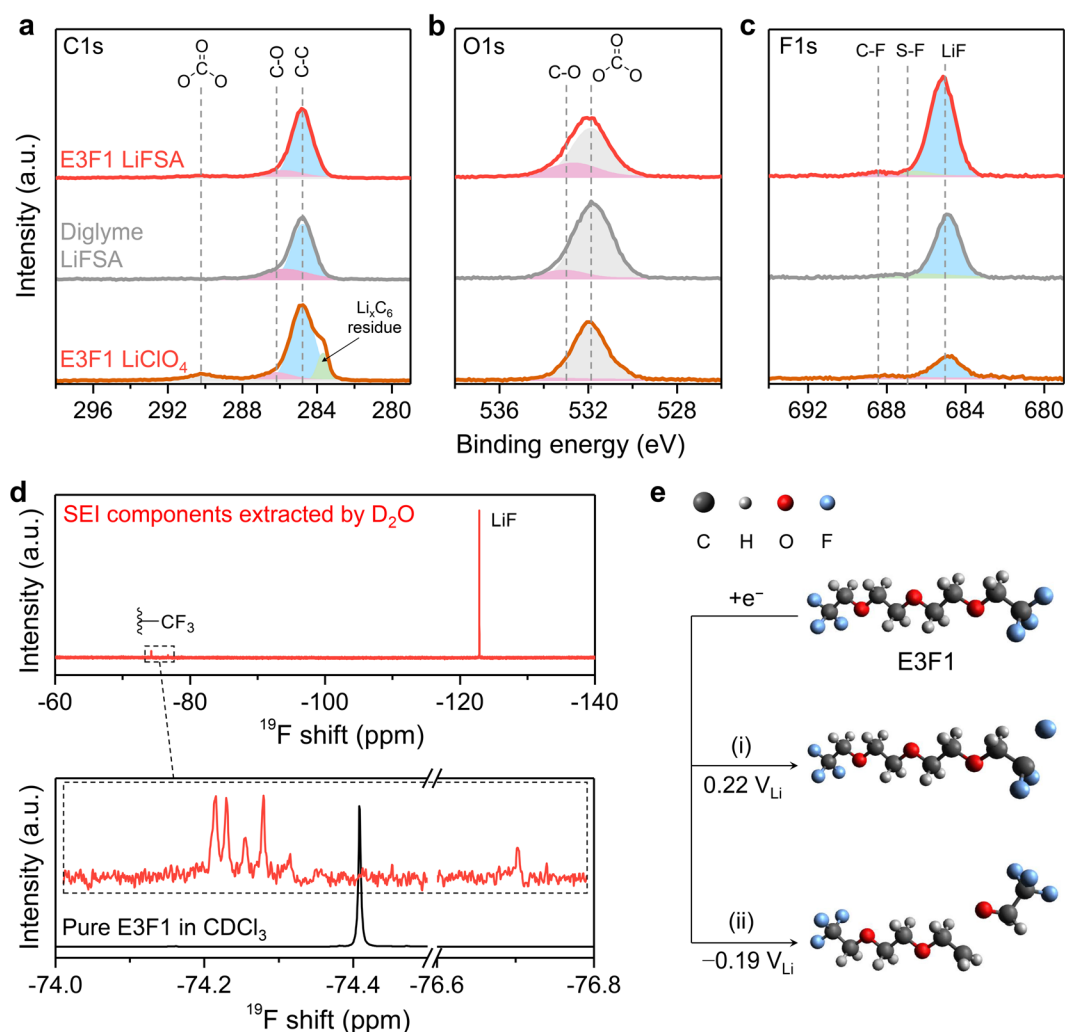
Fig. 6 Interfacial properties. (a–c) XPS of graphite electrodes retrieved from corresponding Gr/Li cells after formation cycles (ending on deintercalation): (a) C1s spectra; (b) O1s spectra; (c) F1s spectra. (d) 19 F NMR spectra of E3F1 1 M LiFSA derived SEI components dissolved in D 2 O. Inset shows an enlarged view of the CF 3 peaks and the 19 F NMR of pure E3F1 in CDCl 3 for comparison. (e) Reductive degradation pathways and corresponding adiabatic reduction potentials of E3F1 predicted by DFT calculations ( V_{\text{Li}} : volts versus Li/Li + ).
