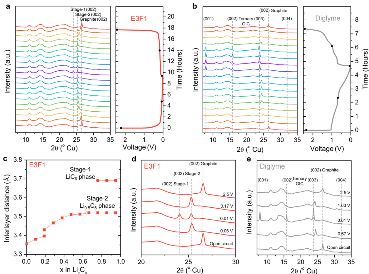
Fig. 4 In situ synchrotron X-ray diffraction (XRD). (a and b) Time-aligned XRD patterns and voltage profiles of Li/Gr cells using (a) 1 M LiFSa in E3F1 and (b) 1 M LiFSa in diglyme as electrolytes. (c) The evolution of graphite interlayer distance when graphite is lithiated in E3F1 electrolyte. (d and e) Enlarged view of XRD patterns at selected points of cycling (marked by black dots in a and b). The cells were cycled at a current rate of C/10 while XRD patterns were collected.
