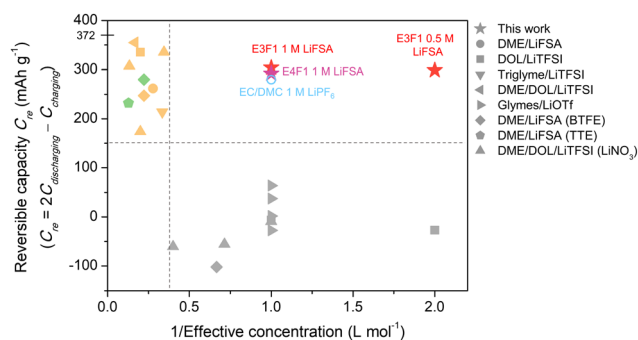
Fig. 7 Comparison of ether electrolytes for lithium-ion batteries. Fluoroethers studied in this work are the only group of ether solvents that can achieve high performance with graphite anodes at conventional salt concentrations. Most normal ether electrolytes with conventional salt concentrations show poor performance with graphite (grey color symbols). High (effective) salt concentrations are required for ether-based HCEs (yellow color symbols) and LHCEs (green color symbols) to enable high reversible capacity. Reversible capacity, defined as 2 \times deintercalation capacity – intercalation capacity, was extracted from data of Li/Gr cells in corresponding references: DME/LiFSA, 19 DOL/LiTFSI, 41 triglyme/LiTFSI, 16 DME/DOL/LiTFSI, 20 Glymes/LiOTf, 14 DME/LiFSA(BTfE) 22 and DME/LiFSA (LiTFSI(LiNO 3 )). 43 To account for realistic solvation structures, effective concentration is defined as molar concentration of salt in the volume of solvating solvent, where non-solvating diluents such as BTfE and TTE are excluded.
