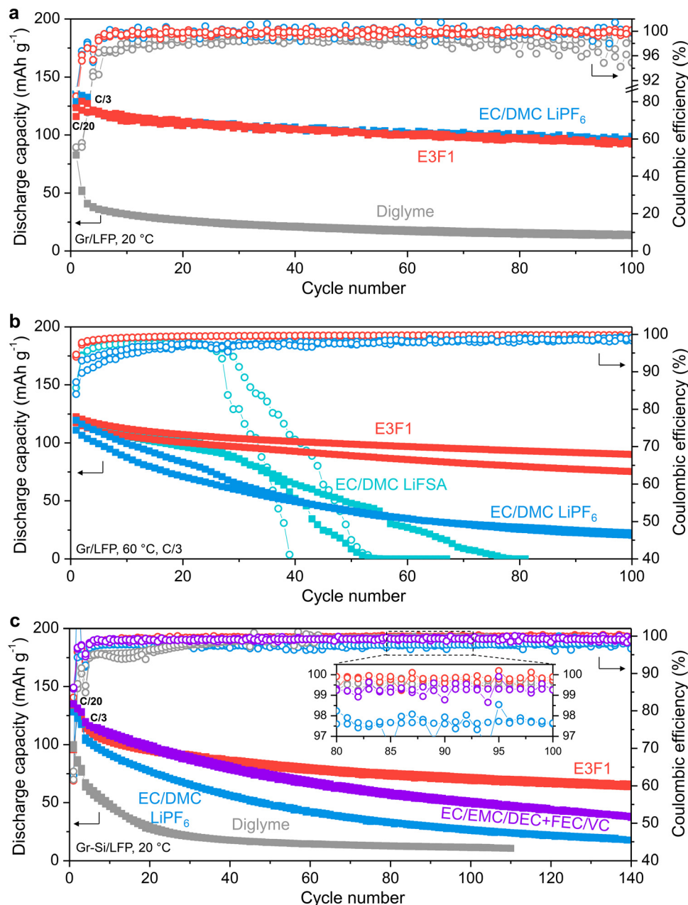
Fig. 5 Cycling performance in full cells. (a) Galvanostatic cycling of graphite/LiFePO 4 (Gr/LFP) full cells at 20 °C using 1 M LiFSA in E3F1 (E3F1), 1 M LiFSA in diglyme (diglyme) and 1 M LiPF 6 in EC/DMC (EC/DMC LiPF 6 ). (b) Galvanostatic cycling of Gr/LFP full cells at 60 °C using E3F1 electrolyte, EC/DMC LiPF 6 electrolyte and 1 M LiFSA in EC/DMC (EC/DMC LiFSA). Three formation cycles at C/20 were performed at 20 °C prior to 60 °C cycling. (c) Galvanostatic cycling of graphite-silicon composite/LiFePO 4 (Gr-Si/LFP) full cells at 20 °C using E3F1 electrolyte, diglyme electrolyte, EC/DMC LiPF 6 electrolyte and 1.2 M LiPF 6 in EC/EMC/DEC + 2% FEC + 1%VC (EC/EMC/DEC + FEC/VC). Two replicate cells of each test are shown. EMC (ethyl methyl carbonate); DEC (diethyl carbonate); FEC (fluoroethylene carbonate); VC (vinylene carbonate).
