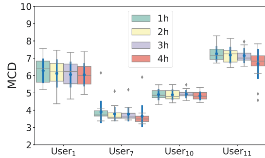
Fig. 20: MCD under the various sizes of the training set
