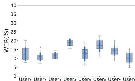
Fig. 11: Word Error Rate based on volunteer recognition for the reconstructed audio
