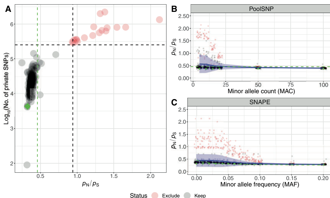
FIG. 2. Quality control of SNPs called with SNAPE-pooled and PoolSNP. Panel (A) shows genome-wide p_N/p_S ratios and the log10-scaled number of private SNPs for all Pool-Seq samples based on SNP calling with SNAPE-pooled. We highlight 20 outlier samples in red, which are characterized by exceptionally high values of both metrics. The dashed black lines indicate the 95% confidence limits (average + 1.96 SD) for both statistics. The vertical green dashed line highlights the empirical estimate of p_N/p_S calculated from individual sequencing data of the DGRP freeze2 data set (Mackay et al. 2012). The green diamond shows the corresponding value of the DGRP population, which was pool-sequenced as part of the DrosRTEC data set (NC_ra_03_n; Zhu et al. 2012). Panels (B) and (C) show the effects of heuristic MAC and MAF thresholds on p_N/p_S ratios in SNP data based on PoolSNP and SNAPE-pooled, respectively. Blue lines in both panels show average genome-wide p_N/p_S ratios across 271 and 246 populations, respectively. The blue ribbons depict the corresponding standard deviations. The 20 outlier samples, which are characterized in panel (A), are highlighted red. In addition, p_N/p_S ratios of the DGRP Pool-Seq sample (NC_ra_03_n) are shown at different cut-offs as green diamonds and the empirical values from the DGRP freeze2 data set are indicated as dashed green lines.
