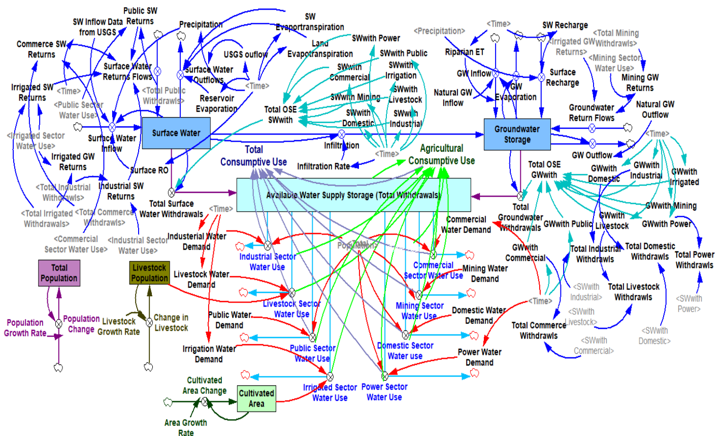
Figure 4. Stock and flow diagram (SFD) used to create the SE-NM model [SFD's parameter details summary is explained in Appendix A, where SW with: Surface Water Withdrawal; GW with: Groundwater Withdrawal].
