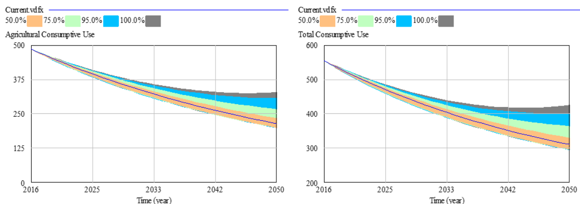
Figure 8. Monte Carlo sensitivity analysis results under livestock change rate.
