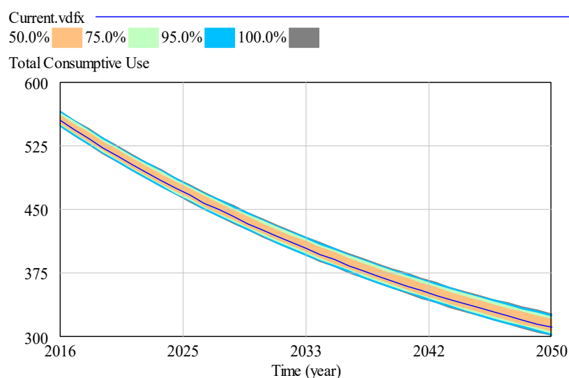
Figure 9. Monte Carlo sensitivity analysis results under mining water demand.
