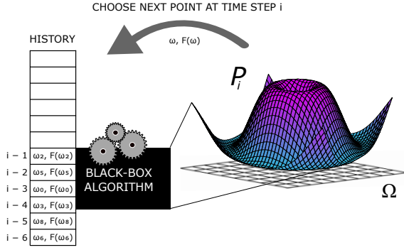
Figure 1: Black-box search algorithm. At time i the algorithm computes a probability distribution P_i over the search space \Omega , using information from the history, and a new point is drawn according to P_i . The point is evaluated using external information resource F . The tuple (\omega, F(\omega)) is then added to the history at position i . Note, indices on \omega elements do not correspond to time step in this diagram, but to sampled locations.
