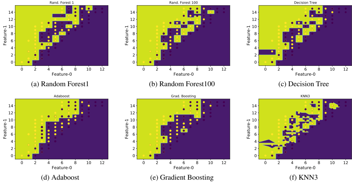
Figure 5: Example decision boundaries for two selected features for axis-aligned algorithms and KNN3. The data is generated using the first two features (x and y position of the box bounding the handwritten letter)
