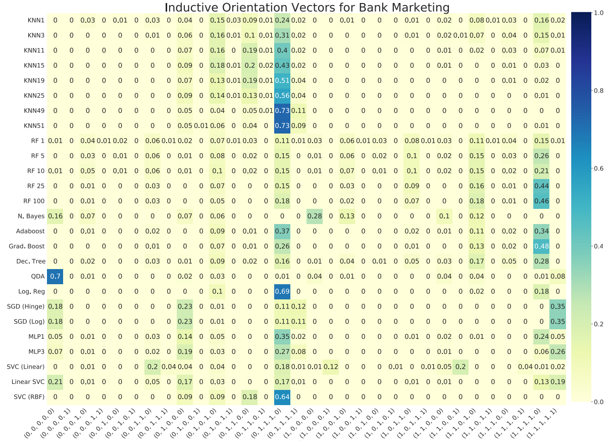
Figure 2: Inductive orientation vectors of algorithms trained on the Bank Marketing Dataset (Note that each 5-tuple corresponds to a particular way of classifying the elements in the holdout set. Each 5-tuple is in the search space \Omega ).
