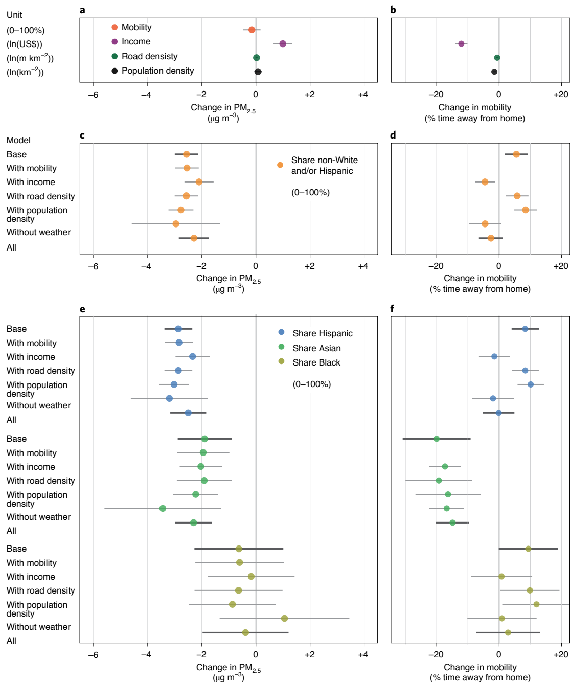
Fig. 3 | Impact of the economic shutdown on (left) PM 2.5 concentrations and (right) mobility. Points show heterogeneous changes across CBG characteristics estimated from difference-in-differences models, along with 95% confidence intervals. Intervals that include zero indicate that there was no differential reduction in exposures across the given gradient. a , Changes in daily PM 2.5 concentration across the shutdown estimated for various socioeconomic variables. The coefficient for mobility is the estimated difference between 0 and 100% of time spent at home; the coefficients for (ln) income, road and population density each represent the impact of an approximate doubling for each variable. b , Similar estimates with mobility as the dependent variable. c,e , Changes in PM 2.5 concentrations over the shutdown period across different racial and ethnic population shares, estimated with different physical and socioeconomic control variables (labels on left). The coefficients correspond to the expected changes between 0 and 100% population share at the CBG level. See Supplementary Tables 2 and 3 for values. d,f , Similar estimates, but with mobility as the outcome instead of PM 2.5 . Values are given in Supplementary Tables 4 and 5. All four panels compare the post-shutdown difference from 2020 to 2019 to the pre-shutdown difference to account for seasonality. In addition, estimates were weighted to reflect the distribution of incomes, population shares and other location characteristics across all block groups in California and correct for the endogenous sampling of ground station locations (Extended Data Fig. 2b, Methods and Supplementary Information). The ‘Base’ model includes CBG and day-of-year fixed effects, as well as weather controls; other models incorporate the noted controls, or exclude weather, and ‘All’ includes everything.
