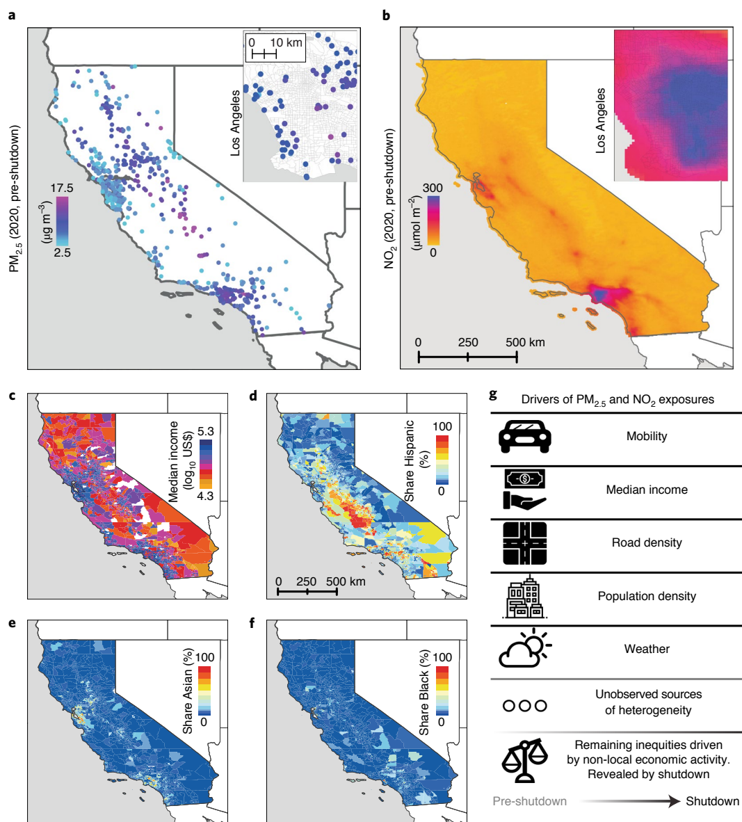
Fig. 1 | Pollution and demographic data used in this study. a,b , Average surface \text{PM}_{2.5} ( a ) and tropospheric \text{NO}_2 ( b ) concentrations in the pre-shutdown period of 2020 in California, United States. c , Median household income (US$) in each CBG from the US Census Bureau 2018 5 yr American Community Survey (ACS). d–f , Share of the population in each CBG that is Hispanic ( d ), Asian ( e ) or Black ( f ), from the ACS. g , Schematic showing both slower-changing (assumed to be static over shorter periods) and higher-frequency factors that contribute to heterogeneous pollution exposures. Symbols in g courtesy of Noun Project: Automobile by Symbolon; Income and Highway by Vectors Point; Urban by Eucalup; weather by asianson.design; List by Richard Kunák; inequality by b farias.
