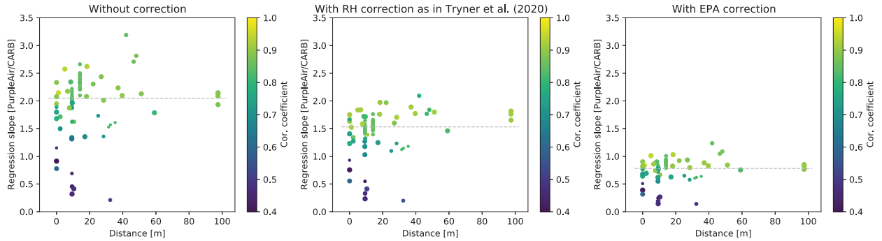
Figure S2: Regression slopes of nearly co-located ( <100\text{m} ) PurpleAir and CARB \text{PM}_{2.5} measurements (2019 and 2020 Jan-Apr outdoor in CA) as a function of distance between the PurpleAir and CARB sensors. Color indicates the correlation coefficient. Marker size indicates the number of points used for the regression. The dashed horizontal line indicates the median. Point size indicates number of points available for the sensor pairs. The three panels show the same comparison with no correction (left), the RH correction proposed in Tryner et al. (2020), and the EPA correction used in the study (right). The RH correction may not be sufficient in our case because we use daily mean data. The EPA correction we implement is conservative. Several PurpleAir sensors are paired with the same CARB sensors (in one case as many as 32). 29 unique CARB sensors are represented here, meaning they have a PurpleAir sensor within 100m. Three sensor pairs were excluded from the figure because the correlation was very low ( < 0.2 ).
