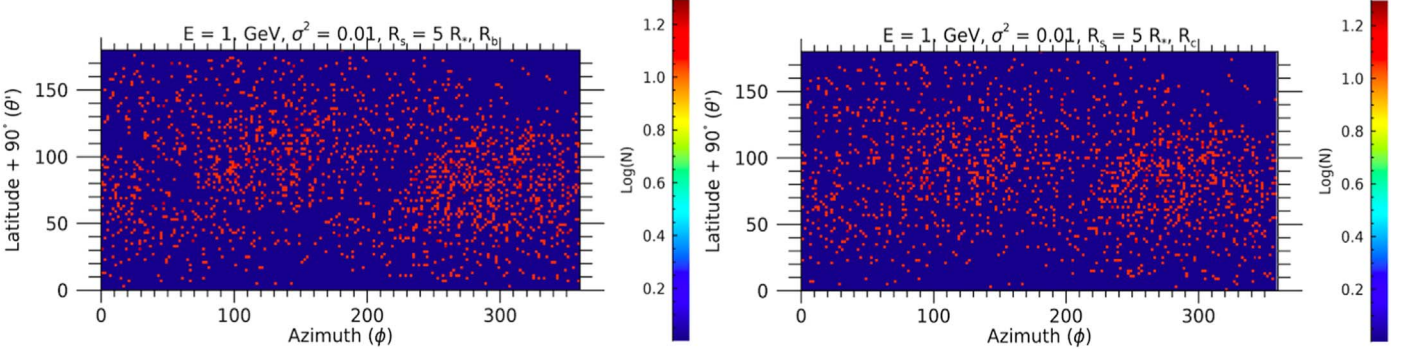
Figure 5. The same as Figure 2 except for a weaker turbulence of \sigma^2 = 0.01 .
