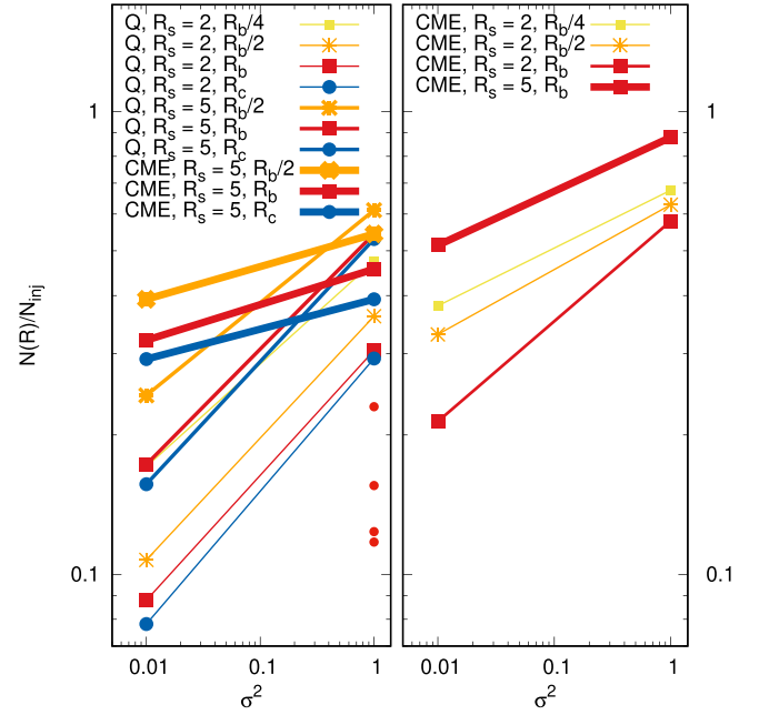
Figure 13. Left: fraction of 1 GeV EPs reaching a given sphere at radius R to the total number of injected EPs, N_{\text{inj}} , as a function of \sigma^2 in the stellar wind reconstructed from the ZDI maps of Klein et al. (2021b). The quiescent case (labeled as “Q”) is compared with the 90 minutes post-CME case (“CME”). The red filled circles refer to the flare case ( R_s = 1.2 R_* ; Figure 7) corresponding, from lowest to highest N(R)/N_{\text{inj}} to R = 0.15 R_b , R_b/4 , R_b/2 , and R_b . Right: same as the left panel but for the stellar wind reconstructed from the ZDI maps of Kochukhov & Reiners (2020), case 1 from (Alvarado-Gómez et al. 2022), in the 90 minutes post-CME case.
