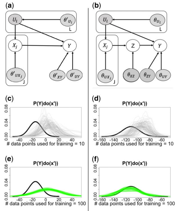
Fig. 2. The estimates of a non-identifiable causal query P_{\mathcal{M}_{\bar{X}}}(\mathbf{Y}|\text{do}(\mathbf{x}')) fail to converge to the true distribution as number of data points used to train the LVM increases (left column). The estimates of an identifiable causal query converge to the true distribution (right column). (a) An LVM where P_{\mathcal{M}_{\bar{X}}}(\mathbf{Y}|\text{do}(\mathbf{x}')) is not non-parametrically identified. Boxes indicate sets of variables with the same structure. Circular white/gray nodes are observed/latent variables. \theta' are model parameters. Each parameter such as \theta'_{U_i} has a prior distribution, e.g., \theta'_{U_i} \sim P(q_{\theta'_{U_i}}) , where q_{\theta'_{U_i}} is a hyperparameter. (b) As in (a), but in this case P_{\mathcal{M}_{\bar{X}}}(\mathbf{Y}|\text{do}(\mathbf{x}')) is non-parametrically identified. (c, e) relate to (a). Thick curve estimates the true distribution P_{\mathcal{M}_{\bar{X}}}(\mathbf{Y}|\text{do}(\mathbf{x}')) , with \theta used to generate interventional data. After training the LVM on N=10 100 observational data points, each thin curve estimates P_{\hat{\mathcal{M}}_{\bar{X}}}(\mathbf{Y}|\text{do}(\mathbf{x}'); \{\mathbf{x}_i, \mathbf{y}_i\}_{i=1}^N, \theta) for each sampled \theta . The curves do not approach the true distribution as number of data points increases. (d, f) relate to (b). The curves converge to the true distribution as the number of data points increases
