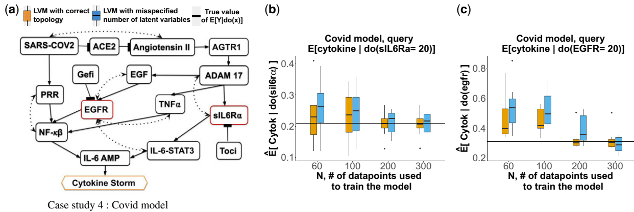
Fig. 6. Synthetic Case Study 4. DAG labeled as in Figure 3. (a) The SARS-CoV-2 model. Dotted edges indicate presence of latent variables. sIL6Rα and EGFR are targets of intervention, Cytokine Storm is the effect. (b) Sampling distribution of \hat{Q}_x = \hat{E}[\text{Cytokine} | \text{do}(sIL6R\alpha = 20)] over 20 observational datasets. (c) As in (b), for \hat{Q}_x = \hat{E}[\text{Cytokine} | \text{do}(EGFR = 20)]
