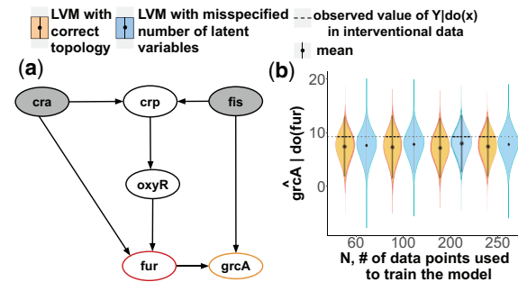
Fig. 8. Experimental Case Study 6. (a) The transcriptional regulatory network with the Napkin motif. (b) The causal query in form of a probability distribution \hat{Q}_{fur} = \hat{P}(grcA | \text{do}(fur) = 0) . The two (overlapping) horizontal dashed lines indicate two observed values of grcA | fur = 0 in the interventional experiments
