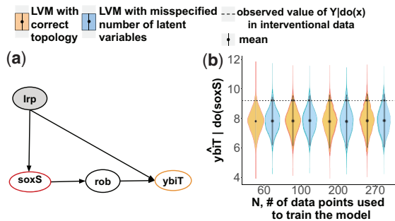
Fig. 7. Experimental Case Study 5. (a) The transcriptional regulatory network with the single-cause feed-forward motif. (b) The causal query in form of a probability distribution \hat{Q}_{soxS} = \hat{P}(ybiT | \text{do}(soxS) = 0) . The two (overlapping) horizontal dashed lines indicate two observed values of ybiT | soxS = 0 in the interventional experiments
