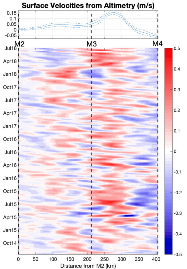
Fig. 7. Hovmöller diagram (bottom) of surface velocities (m/s) from altimetry between OSNAP moorings M2, M3 and M4 over a four-year period (July 2014 – July 2018), with mooring locations denoted by vertical black dashed lines. Positive values are in the prevailing direction of the North Atlantic Current to the north and distances are referenced to mooring M2. Four year mean velocities from altimetry as seen in Fig. 6 are indicated with standard errors (top).
