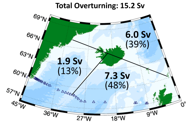
Fig. 10. Summary schematic of overturning in the northern North Atlantic and Norwegian Sea using the isopycnal of maximum overturning along the OSNAP line between Greenland and Scotland ( \sigma_\theta = 27.56 \text{ kg m}^{-3} ). The total in the Iceland/Rockall basins ( 7.3 \pm 2.2 \text{ Sv} ) is the amount determined by this study, the total in the Norwegian Sea is based on historical estimates, and the total in the Irminger Basin in the west is the amount that remains from the total overturning calculation ( 15.2 \text{ Sv} ) as determined by OSNAP. Triangles note the location of OSNAP moorings and bathymetry contours change color with every 1000 \text{ m} in depth.
