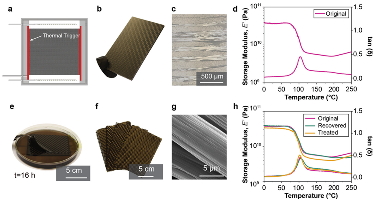
Figure 6. Circular lifecycle of composite materials. a , Schematic representation of fiber-reinforced polymer composites (FRPCs) fabrication through vacuum-assisted resin transfer molding (VARTM) and curing by FP through the thickness by a resistive heater (red). b , Optical image of the resulting FRPC containing a frontally polymerized thermoset containing 10 mol % iPrSi-7. c , Optical micrograph of the FRPC cross-section demonstrating a high fiber volume fraction (ca. 65%) and no void content. d , Representative dynamic mechanical analysis ( 2.0\text{ }^{\circ}\text{C min}^{-1} ) of a frontally polymerized FRPC containing 10 mol % iPrSi-7. e , Chemical deconstruction of the FRPC matrix using 1 M HCl in CPME and f , recovered fabric following deconstruction of the matrix. g , SEM image of the recovered carbon fiber with no evidence of matrix fragments on surface. h Dynamic mechanical analysis ( 2.0\text{ }^{\circ}\text{C min}^{-1} ) of FRPC regenerated from recovered fabric, as well as treated FRPC to simulate environmental weathering compared to the original composite.
