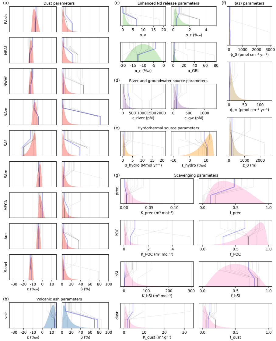
Figure B1. Parameter prior distributions (color-filled densities), and initial and optimized parameter values for a dozen of optimization runs (lines). Each line starts by showing the initial parameter value at the top and is connected to the final optimized value at the bottom. The thicker blue line represents the optimization run that was used as our “best” estimate. (a) Dust \epsilon_{Nd} values ( \epsilon_r ) and solubilities ( \beta_r ) for each region of origin r . (b) Volcanic ash \epsilon_{Nd} value ( \epsilon_{volc} ) and solubility ( \beta_{volc} ). (c) Enhanced Nd release parameters, \alpha curve parameters (curvature \alpha_a and center \alpha_c ), Greenland enhancement ( \alpha_{GRL} ), and global standard deviation of per-grid-cell in situ sedimentary \epsilon_{Nd} ( \sigma_\epsilon ). (d) Rivers and groundwater Nd concentrations ( c_{river} and c_{gw} ). (e) Global hydrothermal source magnitude ( \sigma_{hydro} ) and \epsilon_{Nd} ( \epsilon_{hydro} ). (f) Sedimentary flux parameters ( \phi_0 , \phi_\infty , and z_0 ) (g) Reversible scavenging reaction equilibrium constants, K_X , and fractions returned to water when reaching seafloor, f_X , for each particle type X . See also Table 2.
