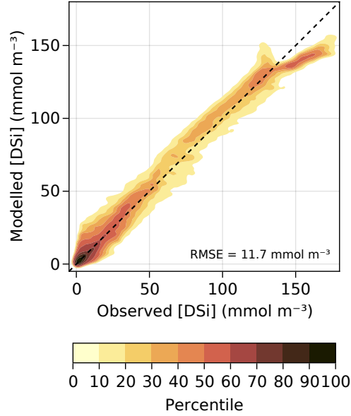
Figure A1. Quantiles of the cumulative joint probability density functions of modelled and observed dissolved Si concentrations for the parallel Si-cycling model. Darker colors indicate high density of data, such that n\% of the modelled and observed data lie outside of the n -th percentile contour. The closer the darker contours are to the 1:1 black dashed line the better the fit.
