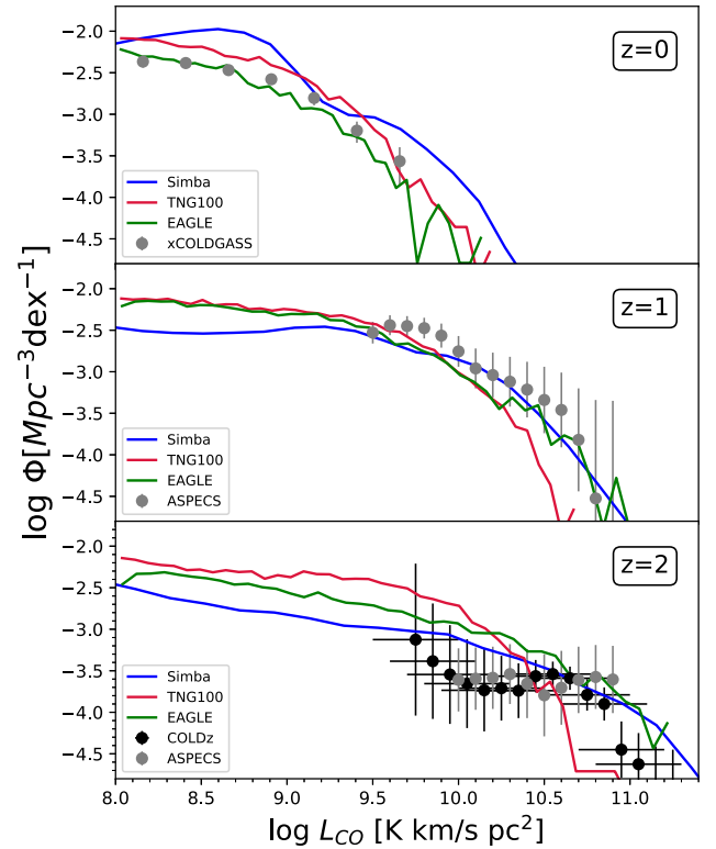
Figure 7. CO(1–0) luminosity functions for SIMBA (blue), IllustrisTNG (red), and EAGLE (green) at z = 0, 1 , and 2 (top to bottom). These are computed using the Narayanan et al. (2012) prescription for \alpha_{\text{CO}} . Observations from xCOLD GASS at z = 0 (Saintonge et al. 2017), ASPECS at z \approx 1 and 2 (Aravena et al. 2019), and COLDz at z \approx 2 (Riechers et al. 2019) are shown in black and grey. IllustrisTNG and EAGLE well reproduce the COLF despite widely different H2MFs, while SIMBA overproduces the COLF like the H2MF. SIMBA and EAGLE are able to reproduce observations of high- L_{\text{CO}(1-0)} galaxies at z \gtrsim 1 .
