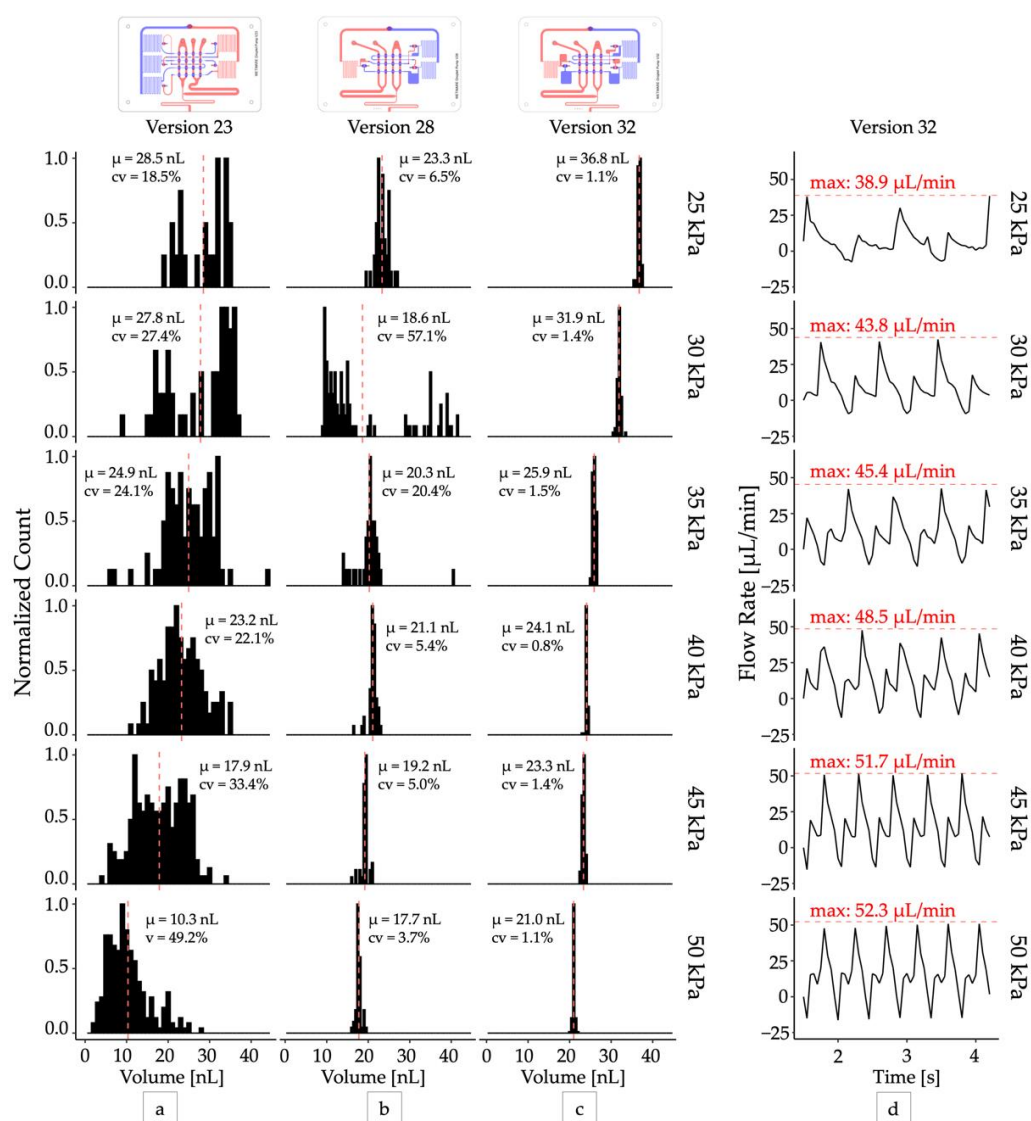
Figure 2. Optimizing droplet monodispersity. Distributions of droplet volumes produced by design iterations (a) Version 23: five-inverter two chamber pump, (b) Version 28: three-inverter single chamber pump with capacitors, (c) Version 32: three-inverter single chamber pump with larger capacitors. All distributions were sampled at steady state with N > 40 . (d) The total output flow rate produced by the optimized droplet generator (version 32). The peak flow rate (red dashed lines) delivered by each pump cycle increased from 38.9 \mu L/min to 52.3 \mu L/min as operating vacuum increased from 25 kPa to 50 kPa.
