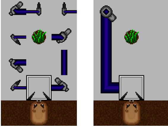
(a) Example of a functional trap generated by the genetic algorithm. (b) Example of a designed trap created by Hom et al.
