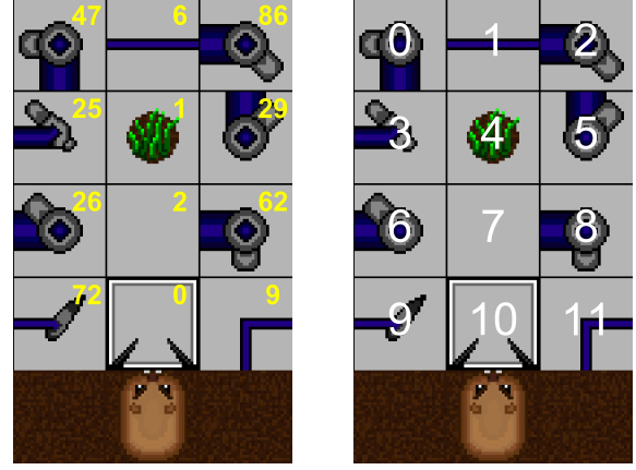
(a) Encodings for 12 trap tiles. (b) Indexing the 12 trap tiles.
