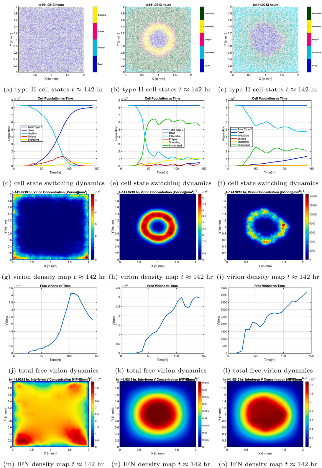
Fig. 8. Effects of IFN-induced paracrine effect. Column 1 has no paracrine mechanism, and it corresponds to the same case and parameters as in first row of Fig. 7 which features the first three combined IFN mechanisms. Column 2 corresponds to having only the fourth IFN mechanism, i.e., the paracrine effect, turned on with parameters J = 0.01 \text{ cell}^{-1} \text{ min}^{-1} [\# \text{ IFN units}]^{-1} \text{ cm}^2 and \tau_4 = 24 \text{ h} . Column 3 features all four IFN-induced mechanisms turned on, combining the scenarios, and combining the same parameters, corresponding to the simulations in columns 1 and 2.
