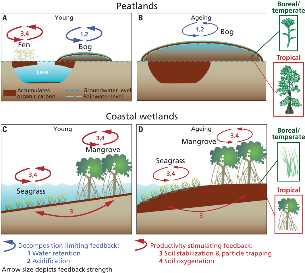
Fig. 2. Conceptual representation of the formation of carbon-storing biogeomorphic wetlands.
