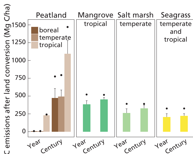
Fig. 3. Carbon emissions after land-use change in biogeomorphic wetlands. Land-use change and (subsequent) chemical and physical erosion result in rapid carbon losses in coastal systems. “Year” indicates 1 year loss. Although carbon losses in peatlands can also be high upon land-use change (for example, logging of tropical forests), they are typically lower but continue for centuries at a slower pace, resulting in higher overall carbon losses. “Century” indicates loss over 100 years. Error bars indicate SD; black dots indicate observed maxima. We assumed instantaneous emissions from biomass after land conversion. For coastal systems, loss of carbon after land conversion was assumed 25 to 100% after year 1 and 63 to 100% after 100 years (74), whereas for peatlands, we applied commonly used land-use emission factors to calculate long-term losses (60, 72). References and methodological details are provided in table S2 (16). [Figure design: Ton A. W. Markus]
