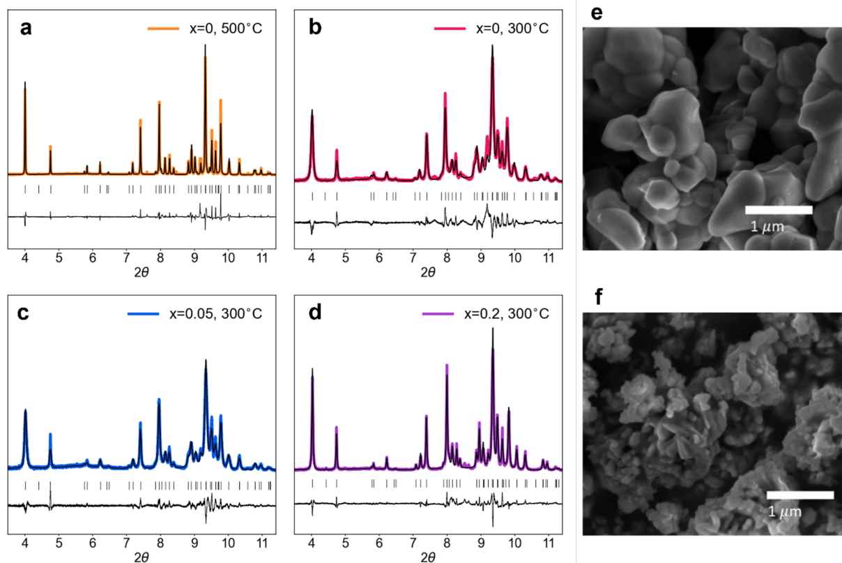
Figure 2. Synchrotron powder XRD patterns collected on a) \text{Na}_2\text{Mn}_3(\text{VO}_4)_3 synthesized at 500°C, and b) \text{Na}_2\text{Mn}_3(\text{VO}_4)_3 , c) \text{Na}_2\text{Mn}_{2.95}\text{Al}_{0.05}(\text{VO}_4)_3 , and d) \text{Na}_2\text{Mn}_{2.8}\text{Al}_{0.2}(\text{VO}_4)_3 synthesized at 300°C. Rietveld refinements and difference curves are shown in black. SEM images of \text{Na}_2\text{Mn}_3(\text{VO}_4)_3 synthesized at e) 500°C and f) 300°C.
