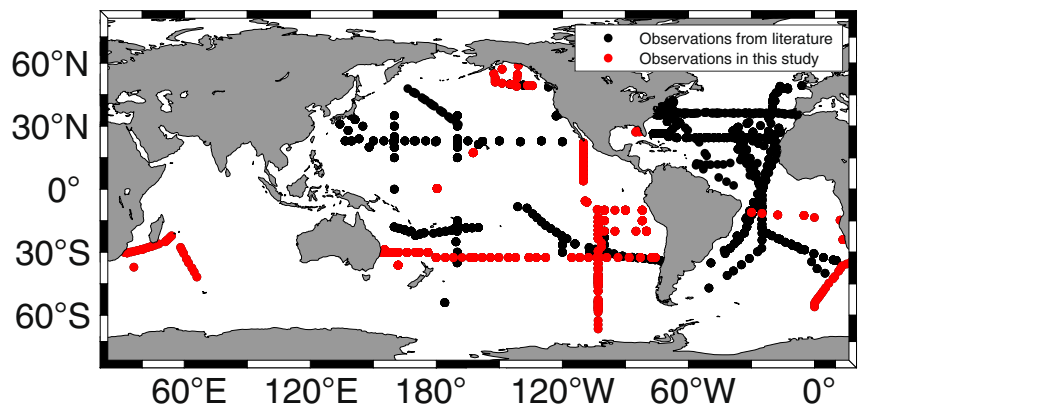
Fig. 1 Global distribution of [DOP] observations in the DOPv2021 database. Black dots represent previously reported data and red dots represent new observations made as part of this study.
