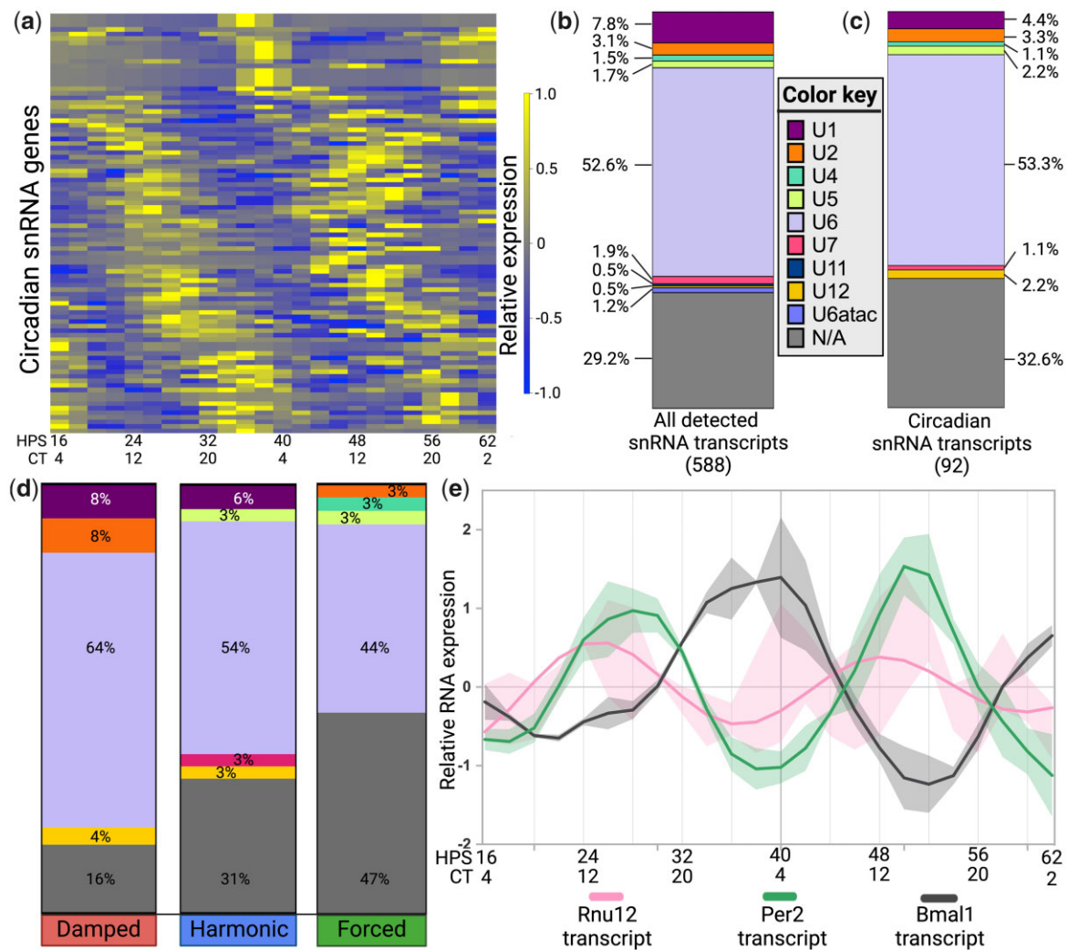
Fig. 5. The circadian clock regulates snRNA expression. a) Heatmap displaying the relative (Z-scored) expression of circadian snRNAs as identified by the PAICE suite (period = 20–28 h, BH-adjusted P -value < 0.05 ). HPS, hours following serum shock for circadian synchronization as in Collins et al. (2021) ; CT, circadian time based on peak and trough Per2 expression of ex vivo peritoneal macrophages as reported in Keller et al. (2009) . b) Bar graph displaying the % distribution of snRNA categories in all detected snRNA transcripts, with gene numbers indicated in parentheses below the bar graph legends. c) Bar graph displaying the % distribution of snRNA categories in all oscillating snRNA transcripts. d) Distribution of oscillating snRNA transcripts across 3 AC categories by snRNA category ( n = 92 total genes, damped n = 25 genes, harmonic n = 35 genes, forced n = 32 genes). e) Expression of ECHO-fitted Rnu12 transcript (period = 23.1 h, BH-adj P -value = 4.18E-4 ), LIMBR-adjusted Per2 transcript (period = 23.1 h, BH-adj P -value = 3.89E-18 ), and Bmal1 transcript (period = 29.3 h, BH-adj P -value = 3.96E-20 ). Dark lines represent the ECHO model while shading represents the standard deviation of the data. The color key references snRNA categories in (b)–(d).
