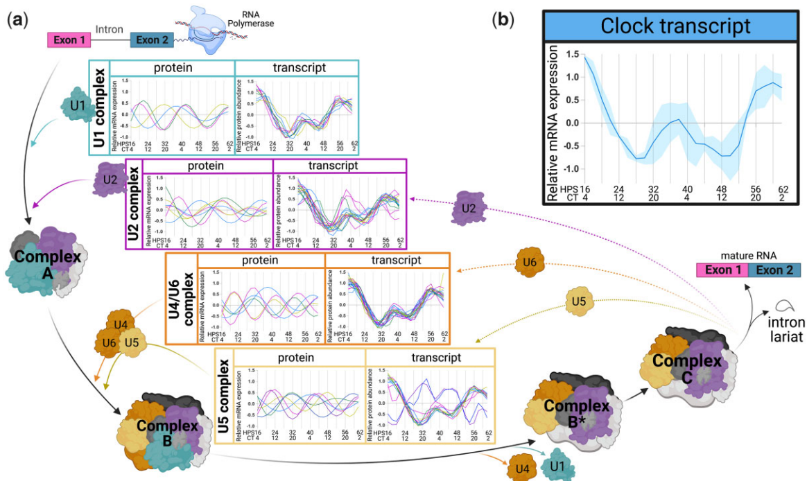
Fig. 6. Circadian oscillations in the transcripts of the components of the spliceosome pathway mirror that of the clock transcript. a) Schematic representation of the canonical spliceosome pathway with the transcripts and proteins in each major complex aligned with the first step in which the complex plays a role in splicing. A newly transcribed pre-RNA binds to members of the U1 and U2 complexes to create complex A. The preassembled U4/U6 and U5 tri-snRNP complexes bind to complex A to create complex B, which, after dissociating from the U1 and U4 complexes, forms activated complex B*. Complex B* and subsequent complex C actively cleave and excise the intron lariat, thereby joining exons 1 and 2 to create the mature RNA, releasing the U2, U5, and U6 complexes, which are recycled back into the spliceosome pathway. The graphs for each major complex (U1, U2, U4/U6, U5) highlight the transcripts and proteins within each respective complex that oscillate with a circadian period, with transcript plots using post-LIMBR data points and protein plots showing ECHO-fitted curves. b) The expression of the clock transcript from the Collins et al. (2021) macrophage data set. HPS, hours following serum shock for circadian synchronization as in Collins et al. (2021); CT, circadian time based on peak and trough Per2 expression of ex vivo peritoneal macrophages as reported in Keller et al. (2009).
