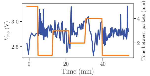
Figure 20: The dynamic sampling rate controlled by the energy-harvesting power supply with changing capacitor voltage over time.
