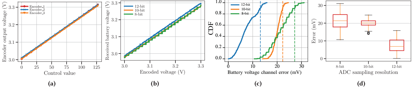
Figure 15: Understanding the effect of different sources of error due to hardware limitations of the design. a) captures the difference in encoder output voltage of three different boards. b) shows that with lower ADC resolution, the number of distinguished voltage levels is reduced, which compromises the bandwidth of the channel. c) and d) characterize the distribution of end-to-end channel error.
