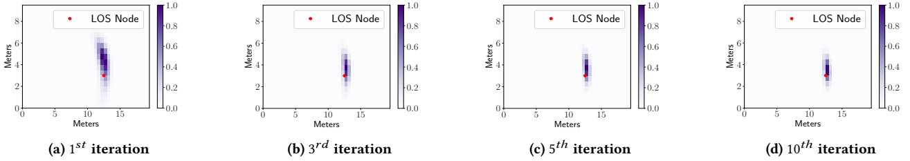
Figure 10: Sampling distribution of estimated target position compared to true location for LOS.
