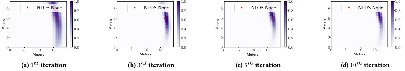
Figure 11: Sampling distribution of estimated target position compared to true location for NLOS.
