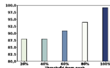
Fig. 16: Declining detection accuracy of KNN classifier was observed with lower cutoff settings
