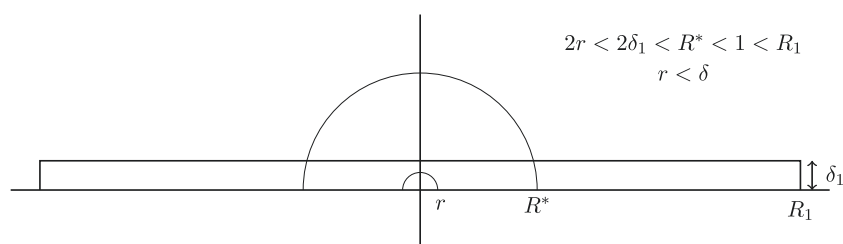
Figure 1. Particle flow around the boundary.
