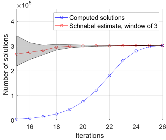
FIGURE 5: Schnabel estimation of the root-count of the polynomial system, window of 3.
