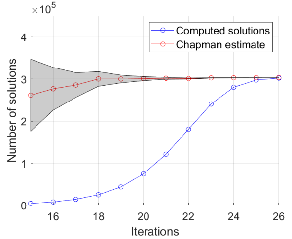
FIGURE 4: Chapman estimation of the root-count of the polynomial system.
