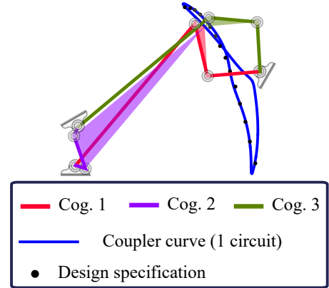
FIGURE 8: A feasible Roberts' cognate triplet, Design III, shown in Table 2.
