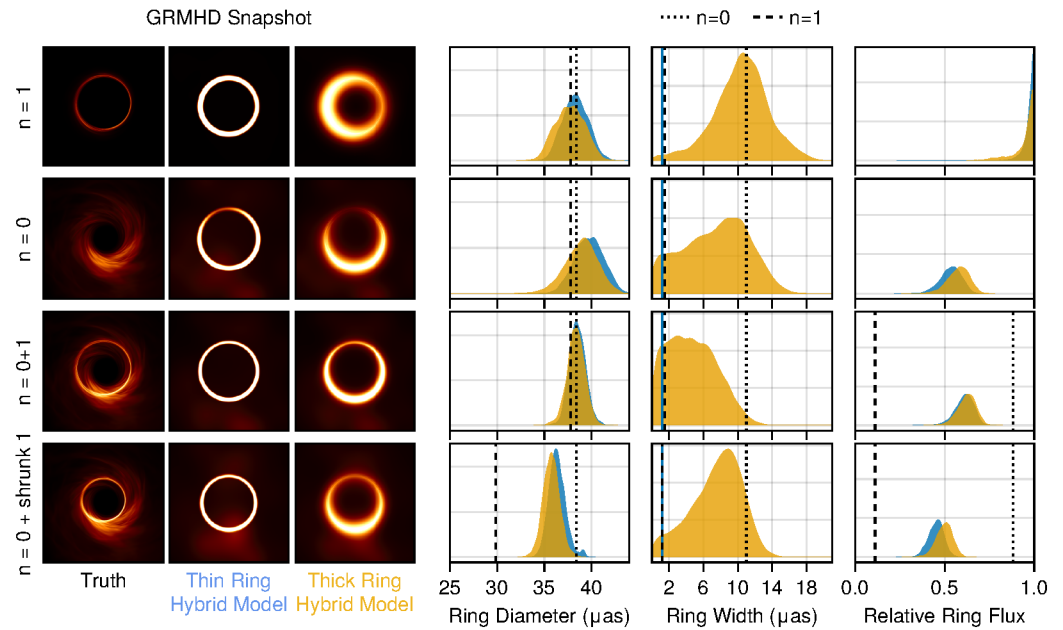
Figure 4. Results of fitting a GRMHD simulation snapshot with coverage corresponding to the EHT 2017 array. The GRMHD simulation has a spin of 0.9375, inclination of 163^\circ , r_{\text{high}} = 10 , and is in the MAD accretion state. The top row shows the results from fitting only the n = 1 emission with the hybrid model, the second row shows fits to only the n = 0 emission, and the third row shows fits to the combined n = 0 + 1 emission. The bottom row shows fits to the combined n = 0 + 1 emission after reducing the diameter of the n = 1 ring by 21%. All rows show both fits that force the ring component to be thin (blue) and fits that do not constrain the ring width (orange). The black dashed lines show true values for the n = 1 photon ring, while the black dotted lines show the true values for the n = 0 photon ring.
