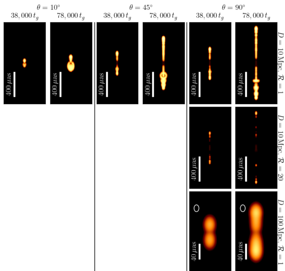
Figure A3. Here we show the full library of base pole images for model m7a0.9-HR. Each image in the top and middle rows spans 1000 \times 1400 \mu\text{as}^2 , and the bottom row spans 170 \times 238 \mu\text{as}^2 . Each image was blurred by convolving the base image with a Gaussian beam with a FWHM of 20 \mu\text{as} (indicated by the white circle in the bottom right panel). The time of each column is indicated at the top; the distance D and plasma temperature ratio \mathcal{R} for each row are indicated on the right. The angle of the observer relative to the jet axis is indicated above each set of two rows. The color scale is logarithmic, spanning three orders of magnitude in each image. We used the same color scale for the D = 10 Mpc images, but reduced the maximum by an order of magnitude in the D = 100 Mpc images to better show the image features.
