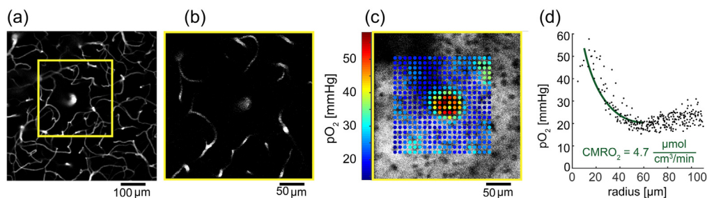
Fig. 32 2P imaging of tissue pO_2 . (a) MIP of a 2P vascular image stack of the top 200 \mu m of cerebral cortex. Contrast is due to intravascular fluorescent dye. (b) Zoomed-in measurement plane. (c) Color-coded pO_2 measurement points overlaid onto the survey phosphorescence image. (d) pO_2 as a function of distance from the center diving arteriole.
