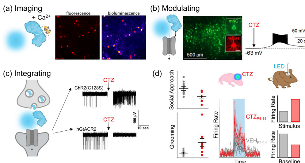
Fig. 16 Bioluminescent tools for imaging, modulating, and integrating. (a)–(c) Luciferases are genetically encoded light emitters that can be employed for imaging neuronal activity when used as a \text{Ca}^{2+} dependent split molecule (a), for modulating neuronal activity when tethered to an optogenetic element (b), and for integrating neuronal activity by expressing the light emitter pre- and the light biosensor post-synaptically (c). (d) Example of experiments taking advantage of the bimodal feature of luminopsins: genetically targeted brain circuits were activated chemogenetically (luciferin) during a defined time window of postnatal development; the same neurons were interrogated in adult animals optogenetically (LED).
