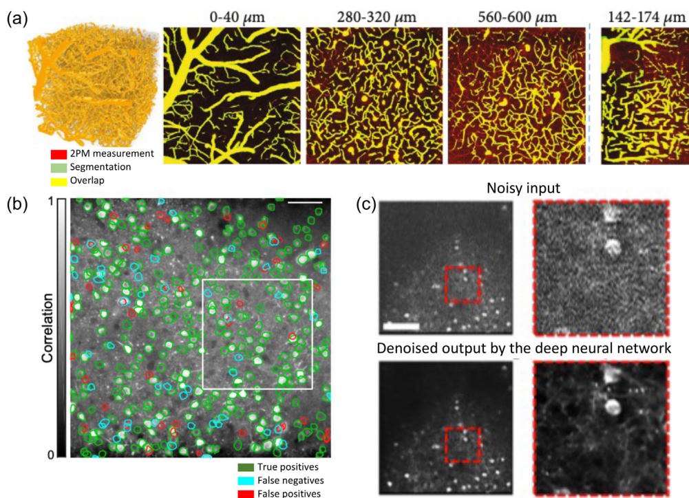
Fig. 40 Deep learning enables state-of-the-art neuronal signal extraction. (a) Vascular segmentation from 2P imaging data. 694 (b) Active neuron segmentation in 2P Ca 2+ imaging. 696 (c) Denoising 2P Ca 2+ imaging data. 697
