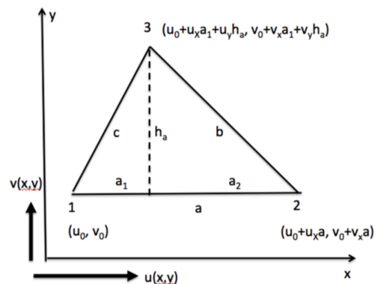
Figure 4. Uncertainty of divergence for a triangle in a spatially varying velocity field with gradients u_x , u_y , v_x , v_y . The height h_a is 2A/a ( A can be calculated from Heron's formula), and a_1 = c^2 - h_a^2 . Side a is the base of the triangle.
