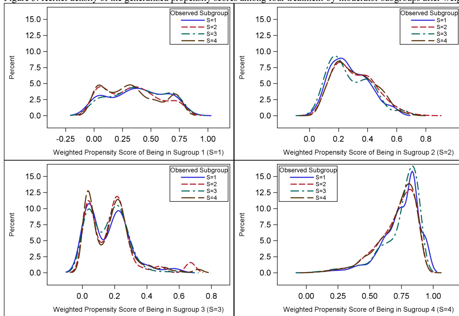
Figure 3: Kernel density of the generalized propensity scores among four treatment-by-moderator subgroups after weighting
