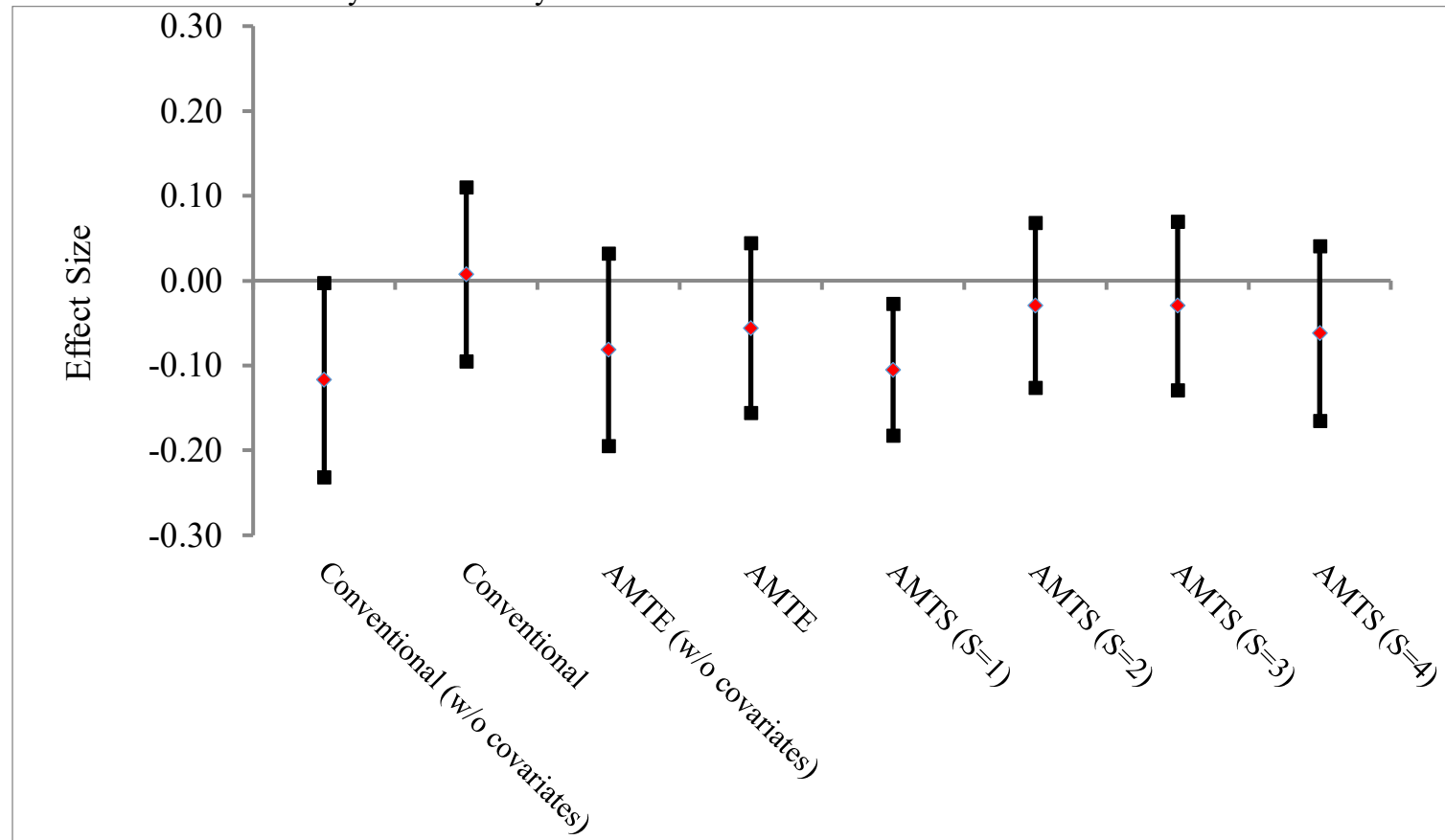
Figure 6: Moderator effect sizes (preschool effect size differences between students speaking and not speaking English at home) and 95% confidence intervals by different analysis
