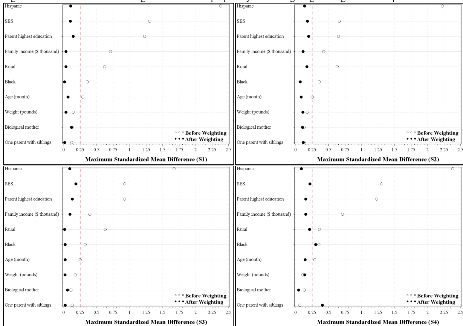
Figure 5: Covariate balance checking before and after propensity score weighting for targeted subsample
