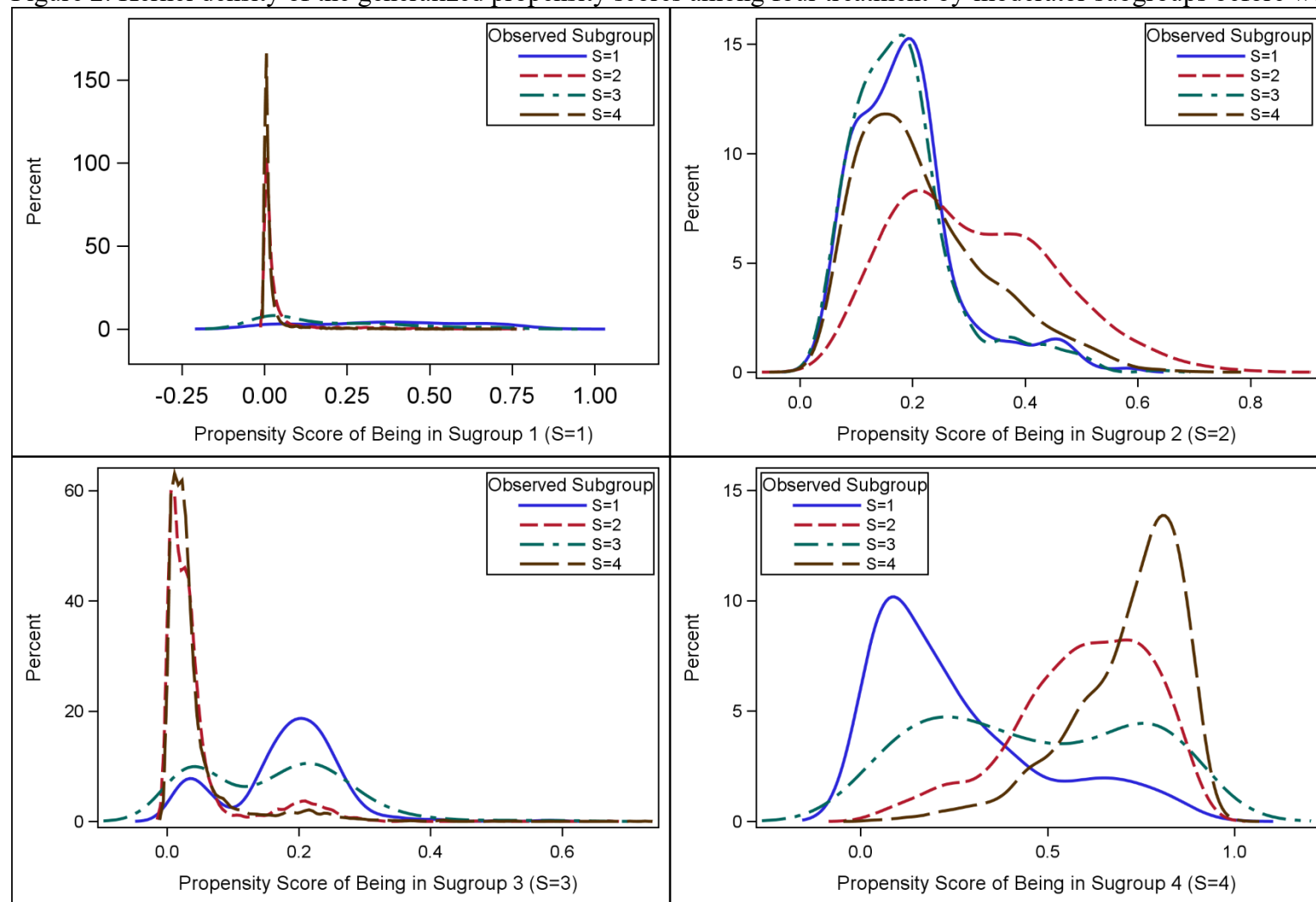
Figure 2: Kernel density of the generalized propensity scores among four treatment-by-moderator subgroups before weighting
