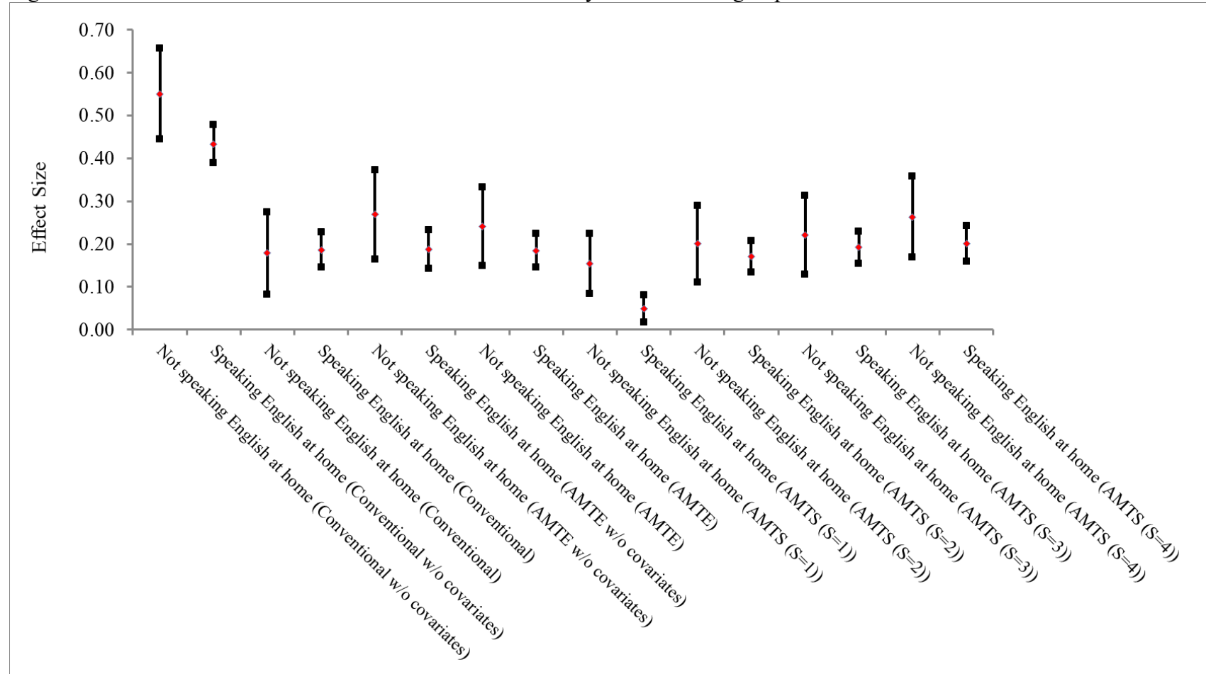
Figure 7: Preschool effect sizes and 95% confidence intervals by moderator subgroups
