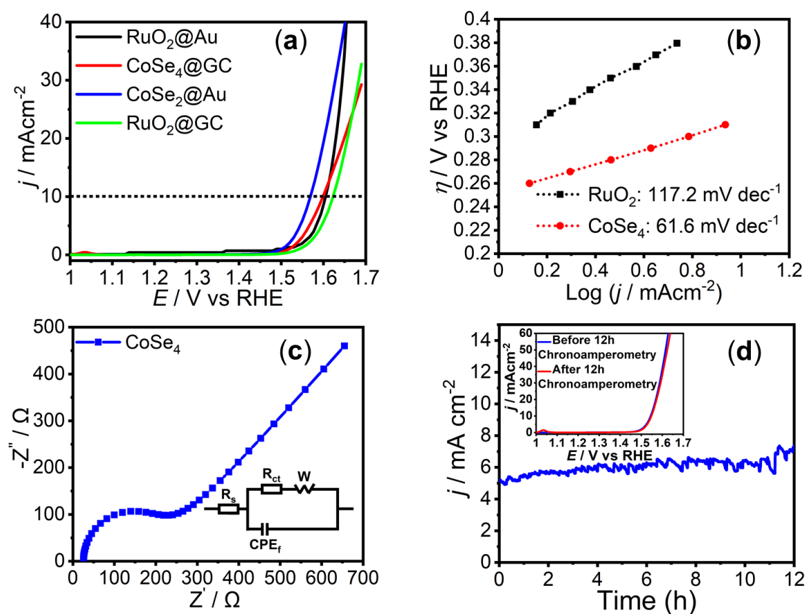
Figure 3. (a) LSV plots of OER for the CoSe 4 catalyst measured in N 2 -saturated 1.0 M KOH solution at a scan rate of 10 mV s -1 . Dashed black line shows the current density of 10 mA cm -2 . (b) Tafel plots of catalysts. (c) EIS spectra measured at 1.56 V vs. RHE in N 2 -saturated 1.0 M KOH solution over the frequency range of 1 MHz to 1 Hz. Inset shows the equivalent circuit where R_s is the electrolyte resistance and R_{ct} is the charge transfer resistance at the catalyst–electrolyte interface. (d) Stability study of CoSe 4 catalyst under continuous O 2 evolution for 12 h at 1.53 V. Inset shows the LSV plots of the CoSe 4 catalyst in N 2 saturated 1.0 M KOH before (blue) and after (red) chronoamperometry for 12 h.
