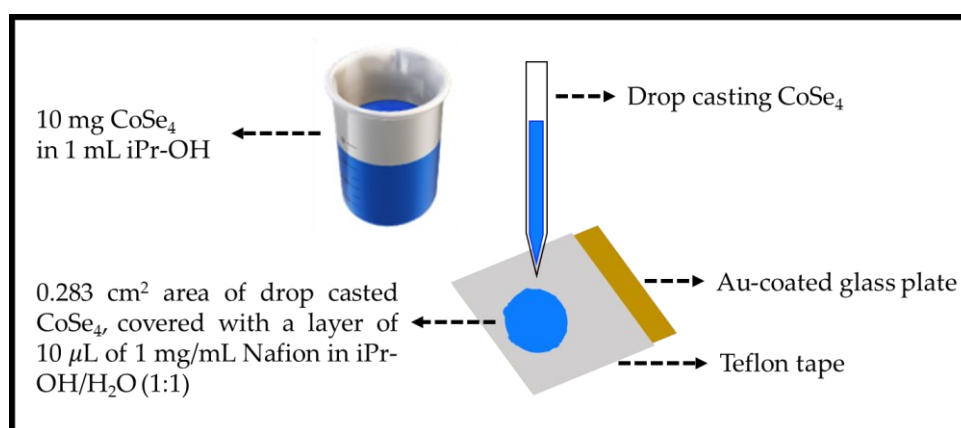
Figure 2. Scheme for electrode preparation.
