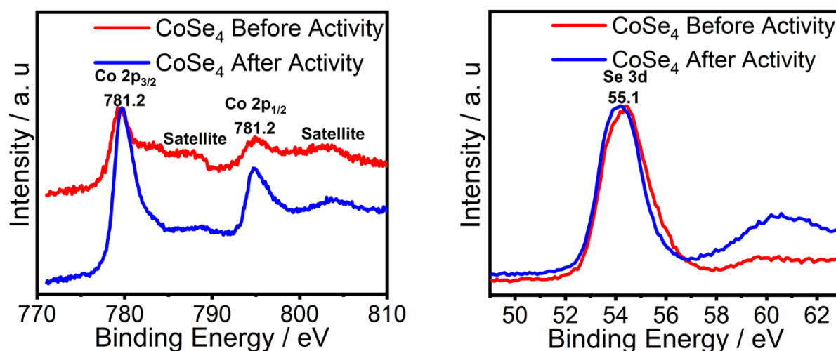
Figure 5. Comparison of XPS peaks of Co 2p and Se 3d before and after OER activity confirming the stability of the \text{CoSe}_4 catalyst.
