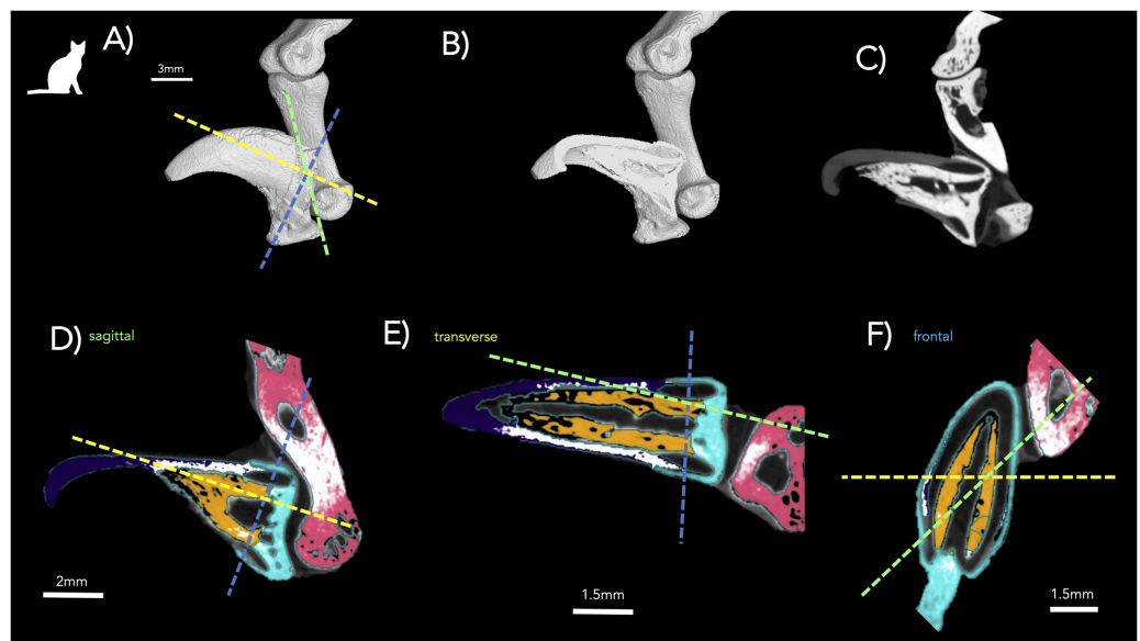
Figure 5 Detailed view \mu CT-scans of cat pes to demonstrate segmentation boundaries. (A) 3D external view of digit IV with colors corresponding to anatomical planes shown in D–F. (B) 3D internal view of 5A; (C) 2D sagittal view of 5B; (D) sagittal segmented structures showing middle phalanx (pink); distal phalanx (teal); bony cap (yellow); and keratinous claw (purple); (E) transverse view of segmenting; and (F) frontal view of claw, where distinct boundaries of the bony cap from the phalanx are visible.
