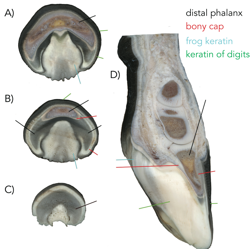
Figure 7 The manus of a fetal horse near full term (A–D). (A) Proximal transverse section showing the frog which are interpreted as parts of digits II and IV. Green pointer shows the wings which are interpreted as digits I and V. Black pointer shows the bone of digit III. (B) Section through the middle of the phalanx. Black pointer shows the bone of digit III, I, and V. Green pointer shows the keratin of digit III. Blue pointer shows the frog which is keratin of II and IV. The red pointer shows the still distinct bone of the bony cap. (C) Distal transverse section showing the bone of digit III (black). (D) Longitudinal section through the manus of the same individual (manus of other side). Black is the distal phalanx of digit III. Red pointers show the bony cap which is intimately congruent to the distal phalanx. Green pointer is the keratin of III. Blue pointer is the keratin of the frog. Full-size DOI: 10.7717/peerj.14352/fig-7
