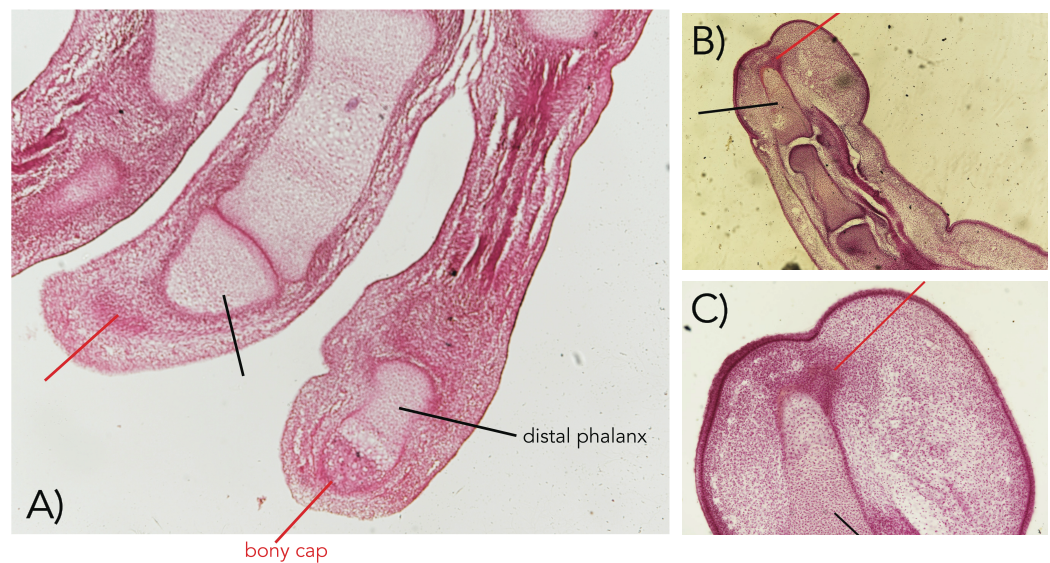
Figure 1 Embryonic human fingers showing the bony cap (A–C). The bony cap in a human from the Carnegie Collection of the Walter Reed Medical Museum (cap marked with red pointer; distal phalanx marked with black pointer). (A) Index and middle fingers from a 22 mm embryo in a longitudinal section (Carnegie Collection stage 22–embryo box number 62, 22 mm). (B and C) Index finger from a 50 mm embryo ventral is to the right, dorsal is to the left (11 weeks; Carnegie Collection embryo box 84 stage 22). Magnification of all 40×.
