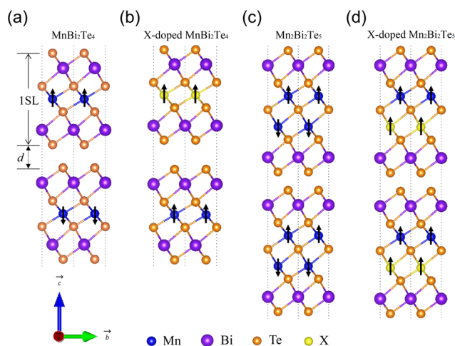
Fig. 1 Crystal structures of layered \text{MnBi}_2\text{Te}_4 (MBT) (a), X-doped MBT (b), \text{Mn}_2\text{Bi}_2\text{Te}_5 ( \text{M}_2\text{BT} ) (c), and X-doped \text{M}_2\text{BT} (d), where X represents transition-metal (TM) dopants. The black arrows denote the directions of the magnetic moments of TMs. Here “ d ” is the interlayer distance.
