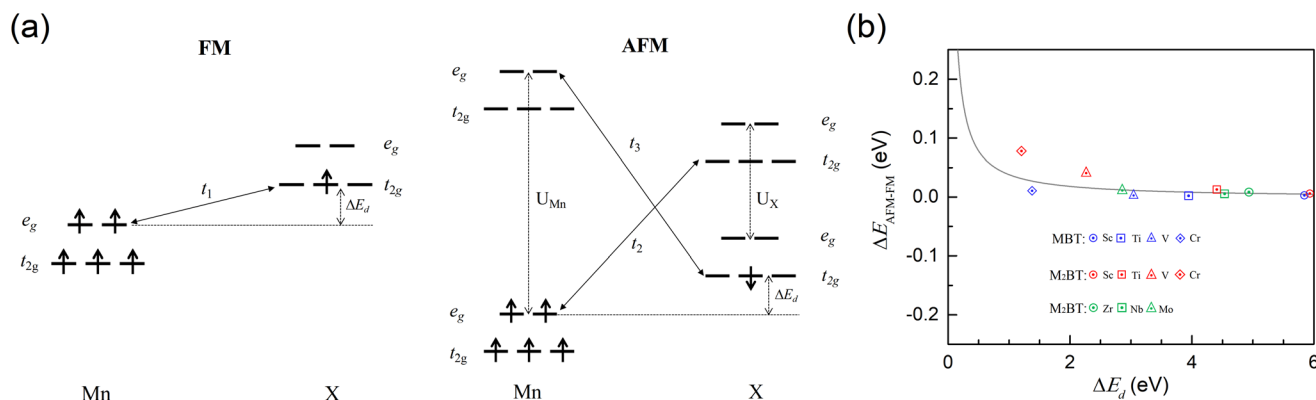
Fig. 2 (a) Schematic diagrams of FM and AFM coupling in X-doped MBTs. (b) The energy difference \Delta E_{\text{AFM-FM}} between AFM and FM phases as a function of \Delta E_d (the relative position of the dopant d- t_{2g} band and the Mn d- e_g band). The parameters are set as: t_1 = 0.1 eV, t_2 = t_3 = 0.05 eV, U_{\text{Mn}} = 9.0 eV, and U_{\text{X}} = 7.0 eV. For comparison, \Delta E_d of X-doped MBTs and \text{M}_2\text{BTs} obtained from DFT calculations is also given.
